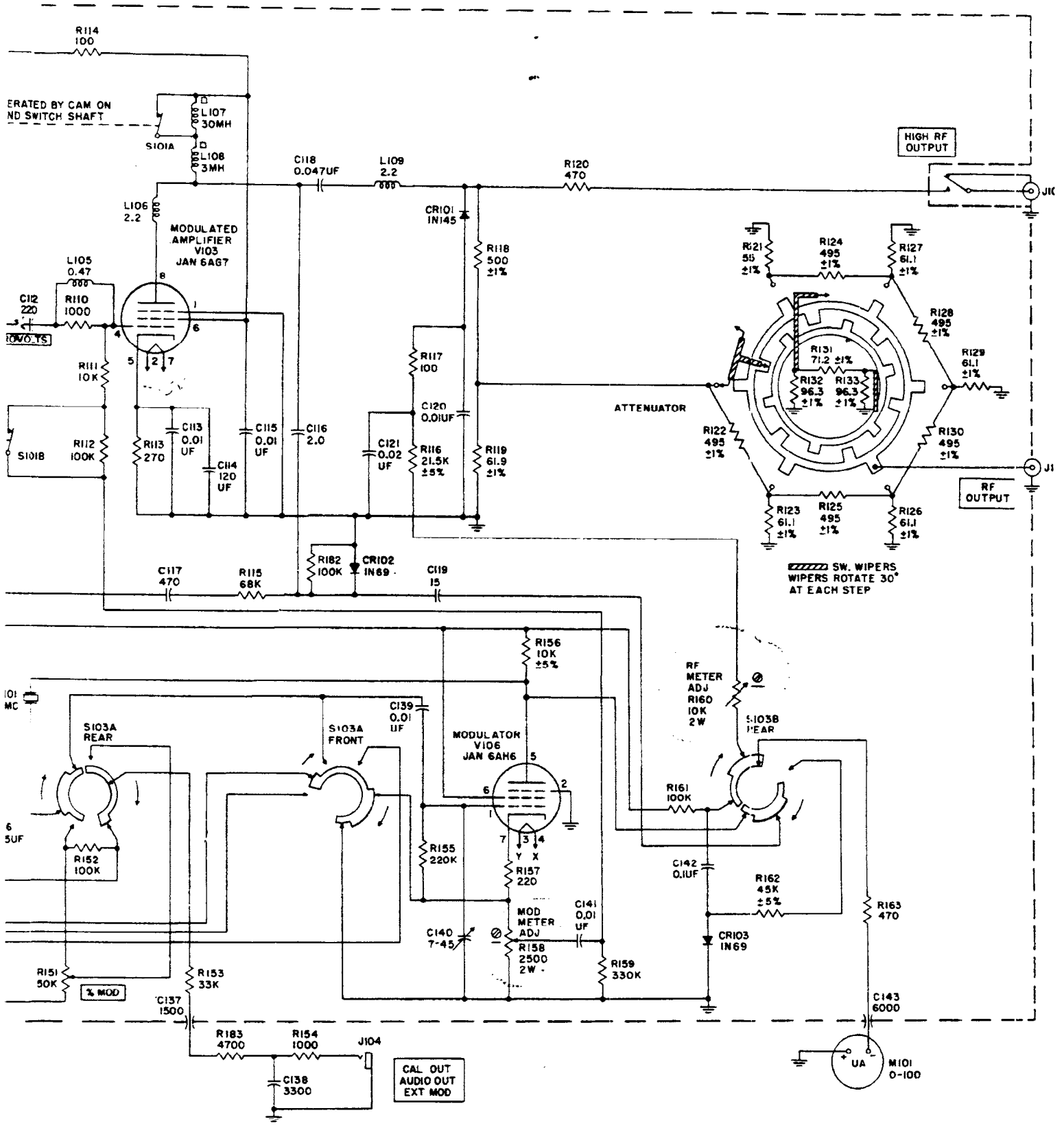
Figure 7-14. RF Signal Generator
