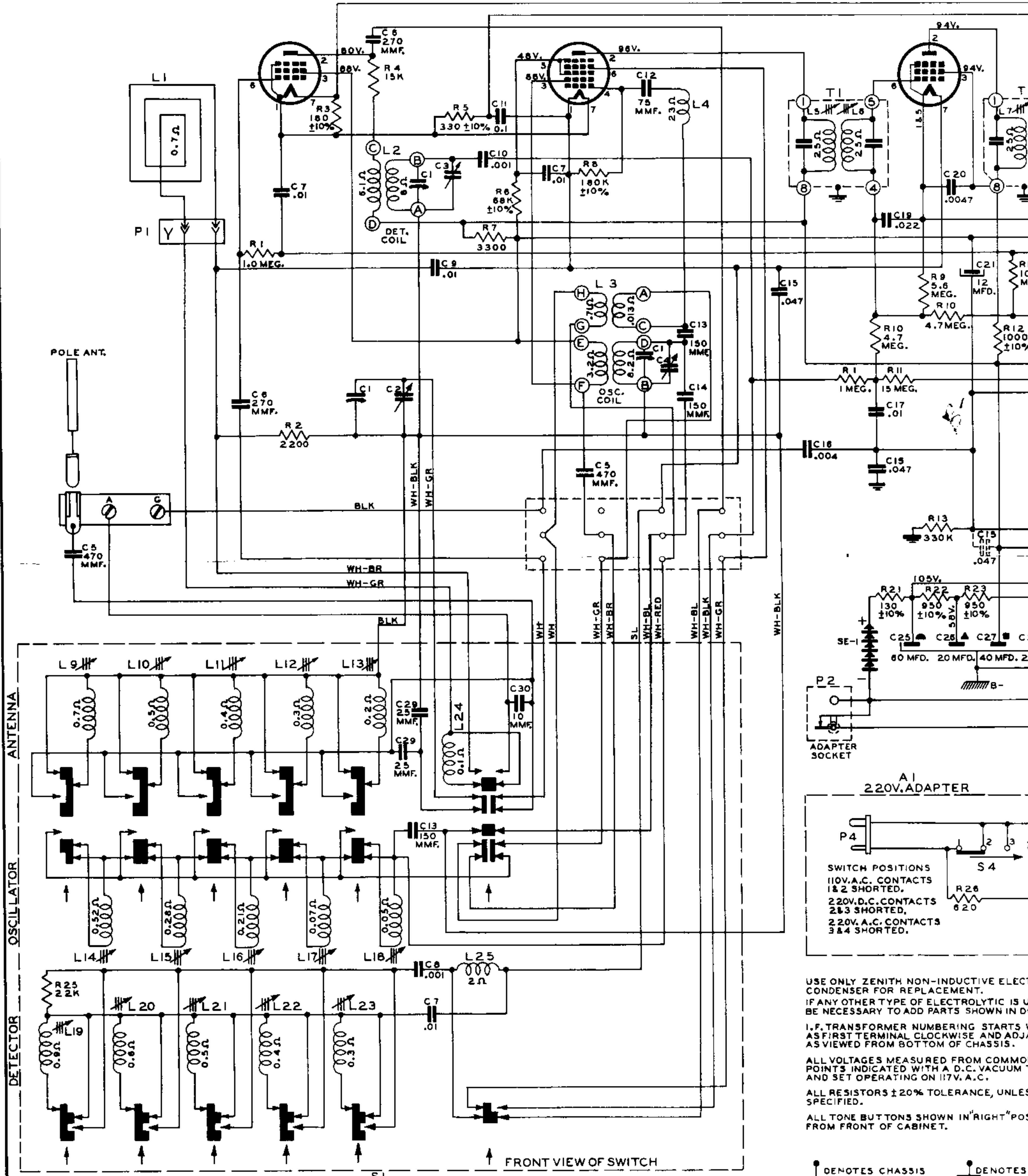
BAND SELECTOR SWITCH, COIL AND WIRE ASSEMBLY BAND SWITCH BUTTONS SHOWN IN NON-OPERATED "OUT" POSITION
