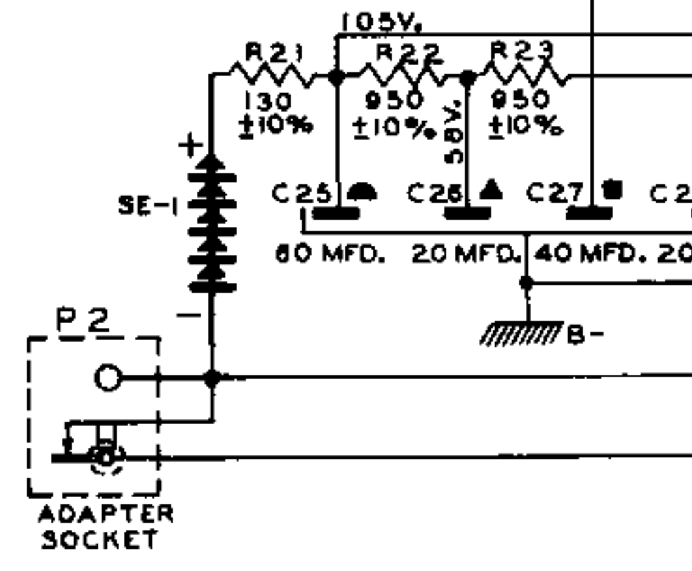
A1 220V ADAPTER SWITCH POSITIONS 110V. A.C. CONTACTS 1 & 2 SHORTED. 220V. D.C. CONTACTS 2 & 3 SHORTED. 220V. A.C. CONTACTS 3 & 4 SHORTED.
