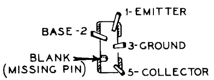
BOTTOM VIEW OF TRANSISTOR SOCKET
