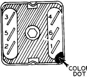
BOTTOM VIEW OF COIL
