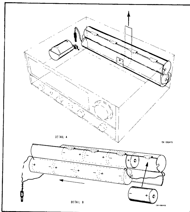
Figure 2. Battery Replacement Detail.
