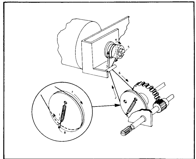
Figure 3. Restringing the Dial Drum.
