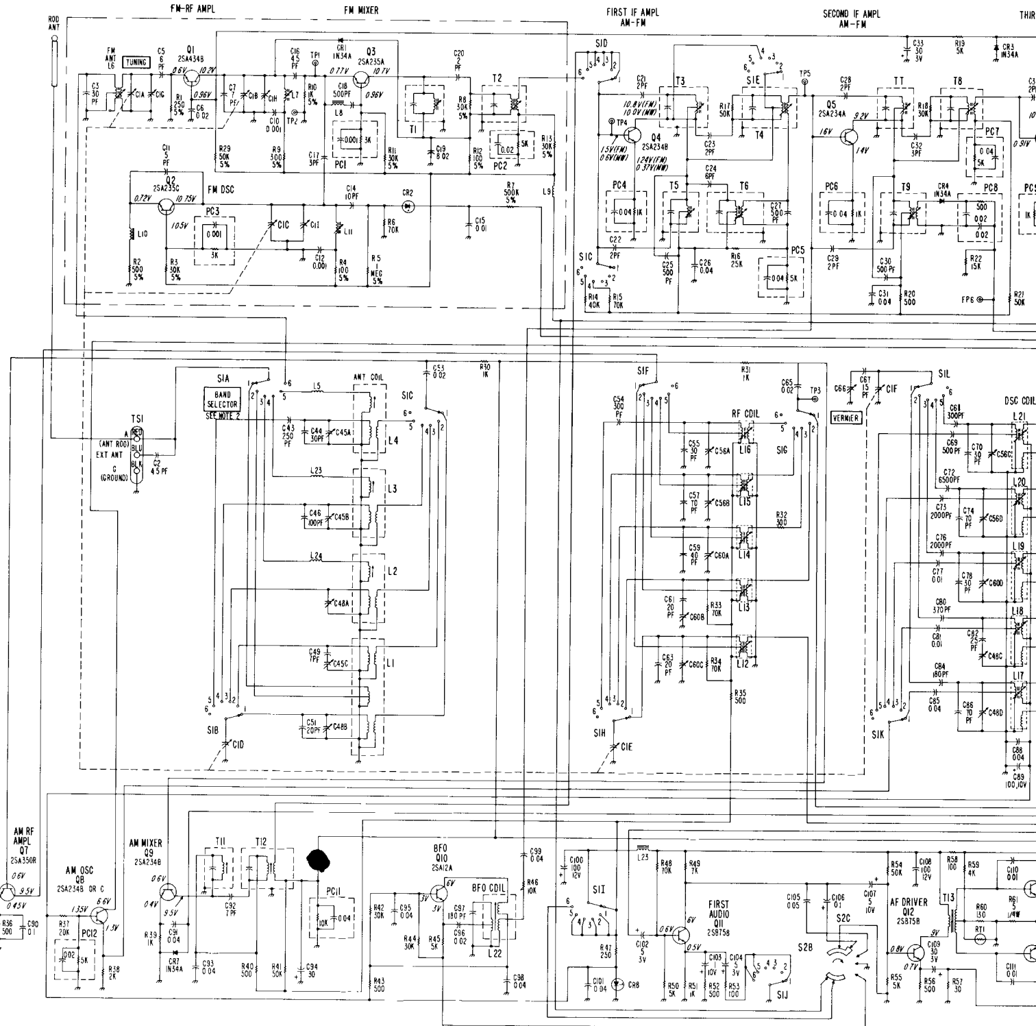
Figure 5. WR-4000 Schematic Diagram.
