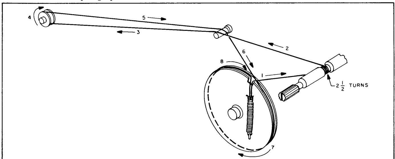
Figure 4. Restringing the Tuning Dial Pointer.
