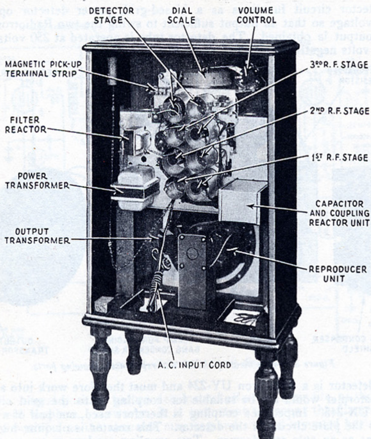
Figure 4—Rear interior cabinet view with shields removed.
