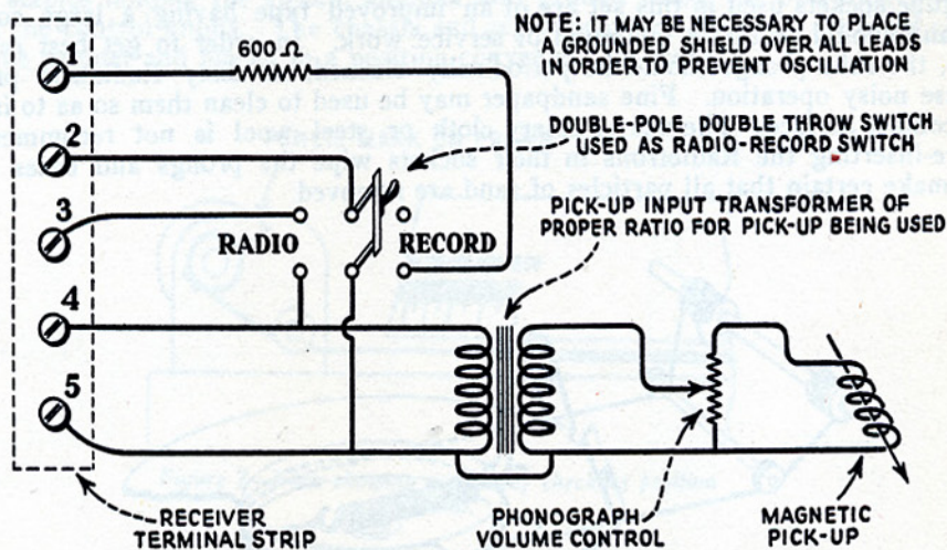
Figure 5—Connections for attaching a magnetic pick-up.
