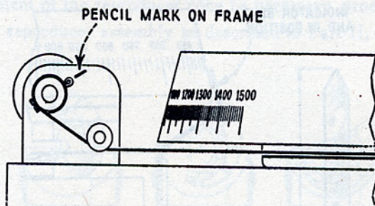
Figure 7—View showing method of checking position of dial.
