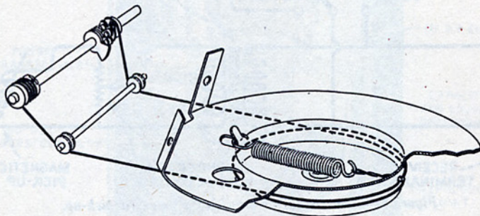
Figure 6—Drive cord arrangement.
