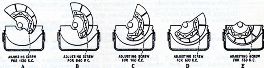
Figure 9—Gang condenser adjustment positions.
