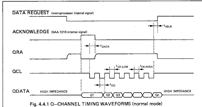
Fig. 4.4.1 Q-CHANNEL TIMING WAVEFORMS (normal mode)
