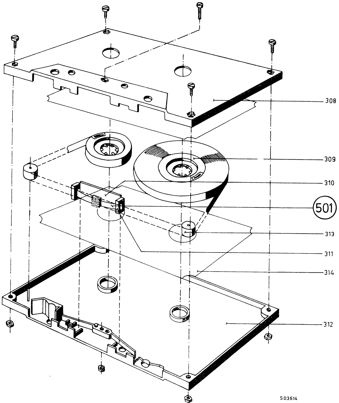
Fig. 13—Cassette Assembly EL1903
