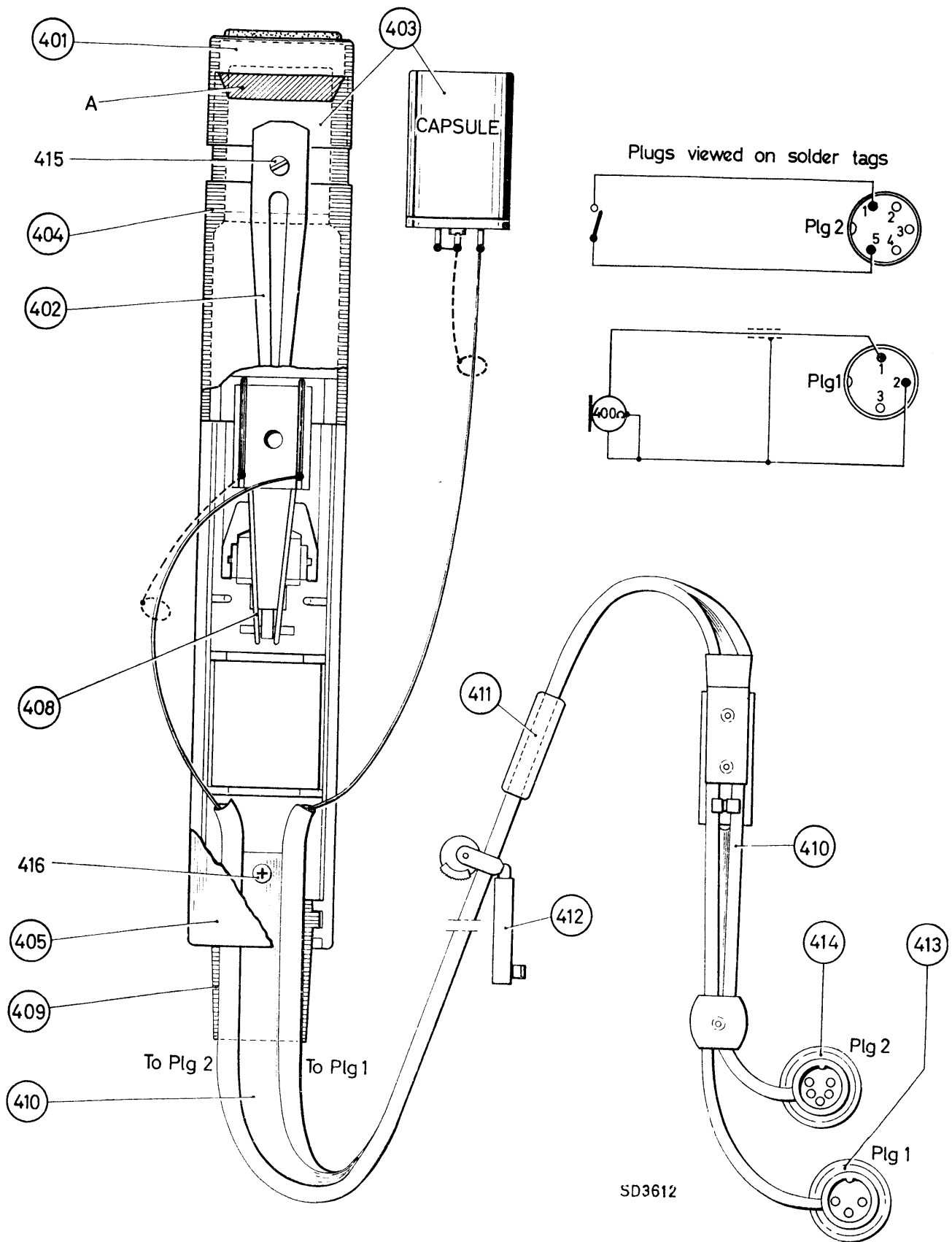
Fig. 15—Microphone and Remote Control Unit—EL1974/13
