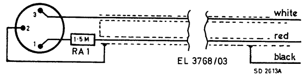
Fig. 3—Radio/Pick-up Connecting Lead
