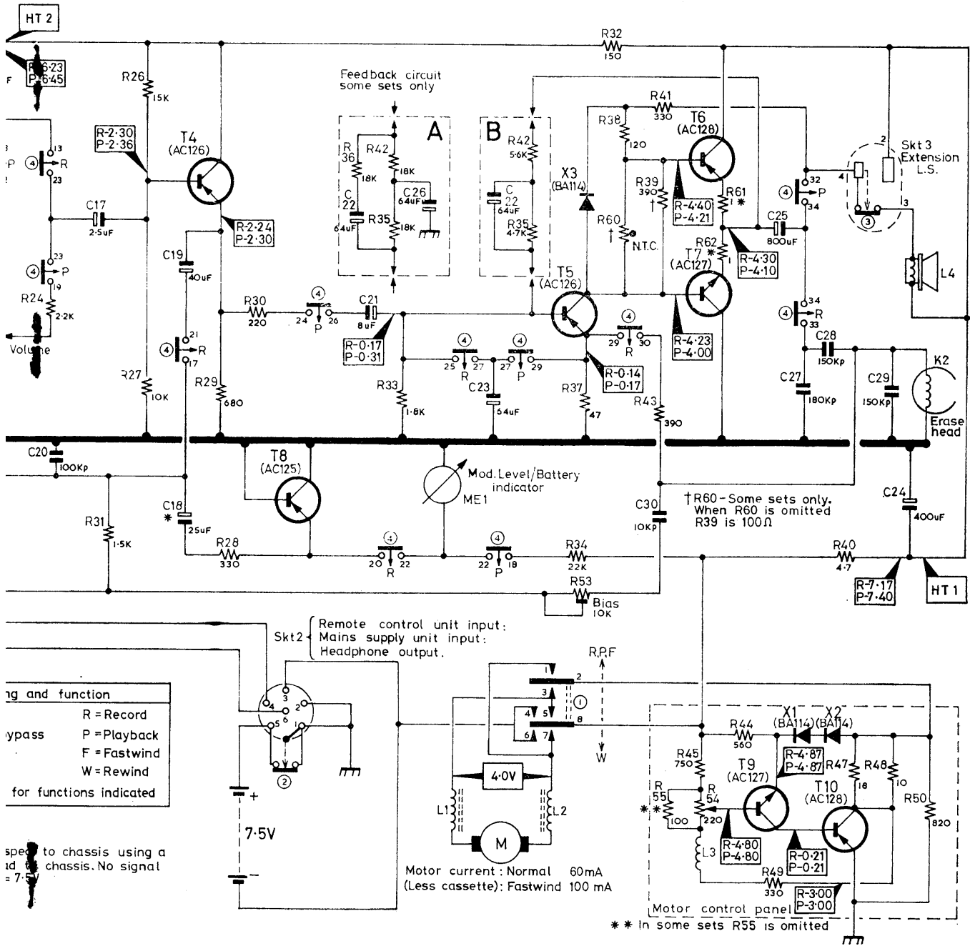
Circuit Diagram
