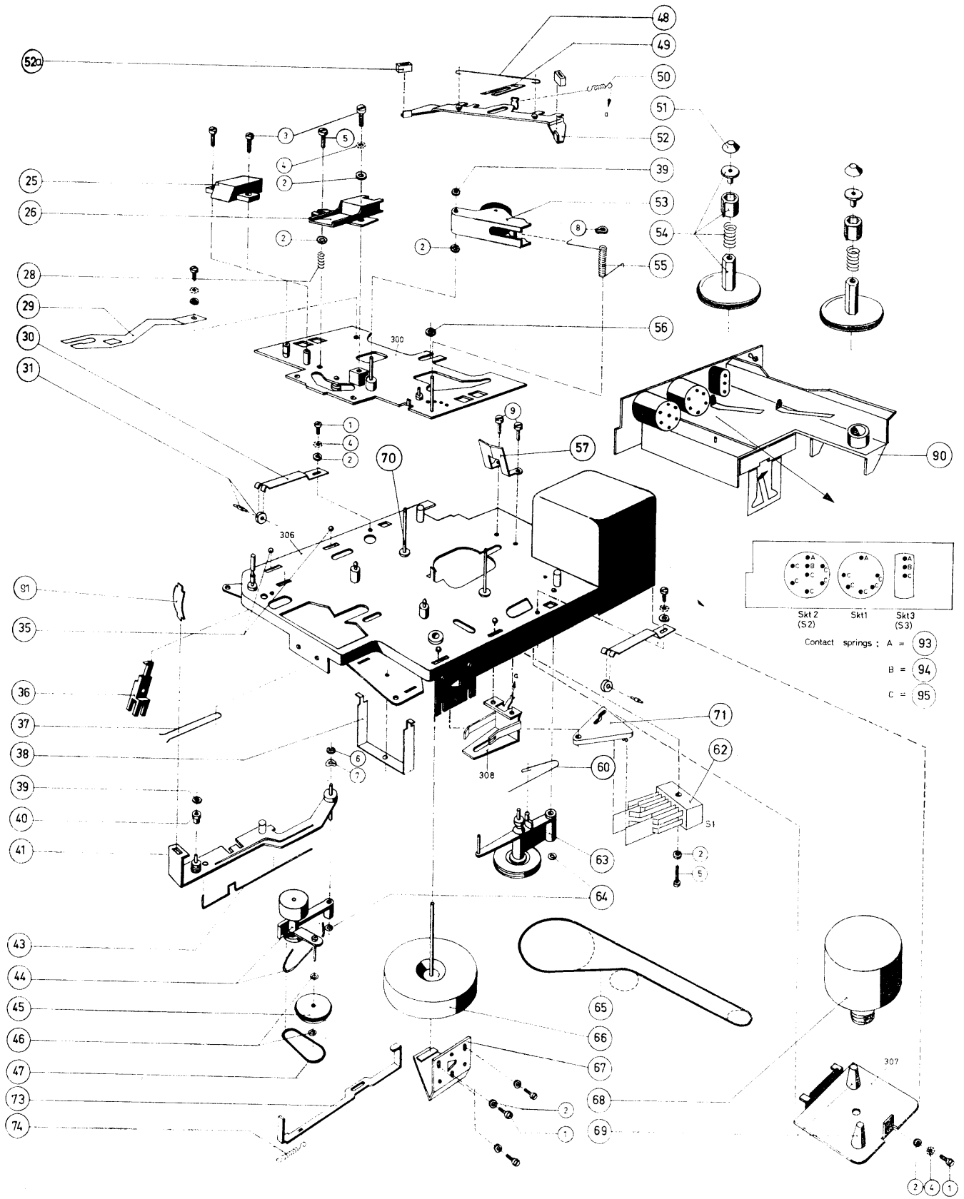
Fig. II—Exploded View
