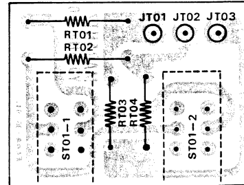
Figure 12. Speaker Switch Assembly PT01 Component Locations
