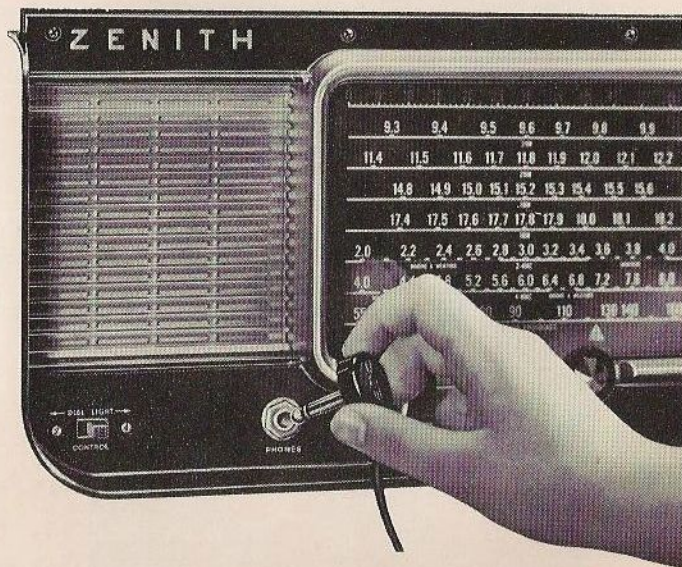
Figure 11—Headphones Connected to Receiver.
