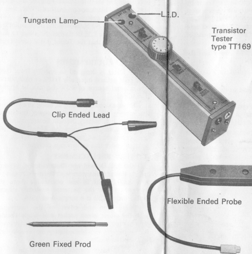
The Transistor Tester with accessories supplied
