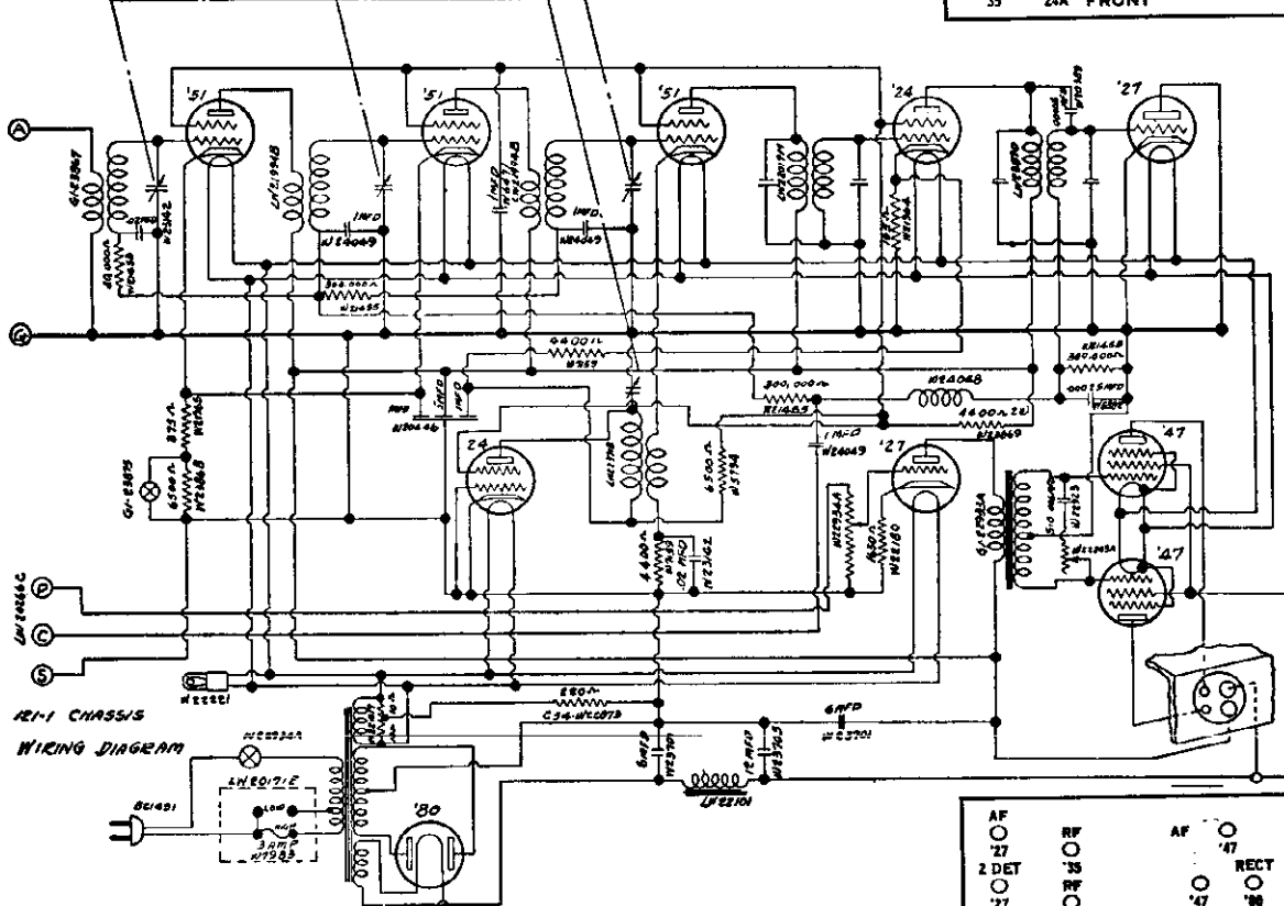
121-1 CHASSIS WIRING DIAGRAM
