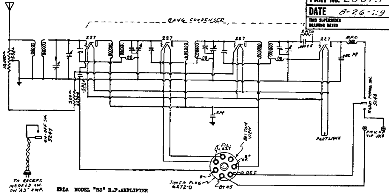
ERLA MODEL "R3" R.F. AMPLIFIER
