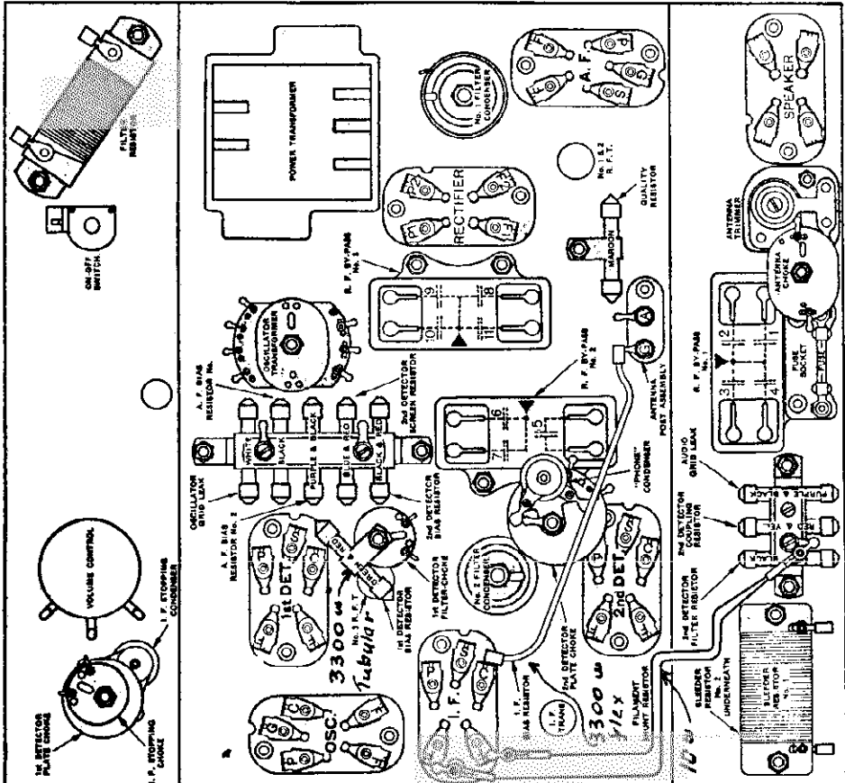
CHART OF EARLY-TYPE MODEL 84, 84-F.
