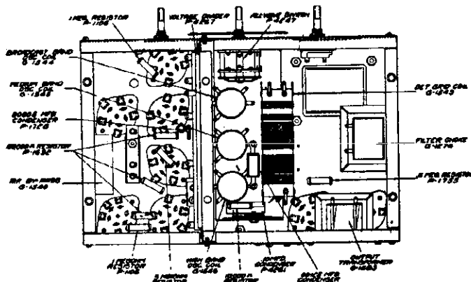
G-240 CHASSIS BOTTOM VIEW
