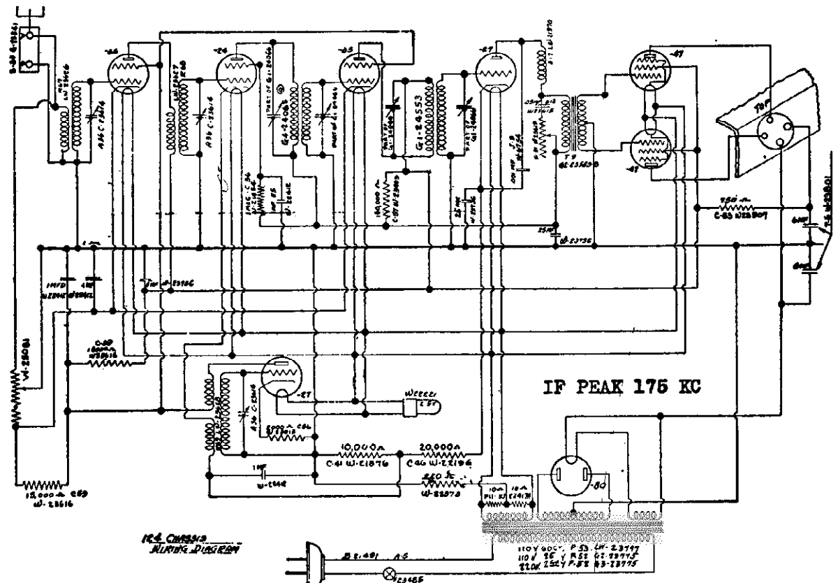
Model 124 Circuit
