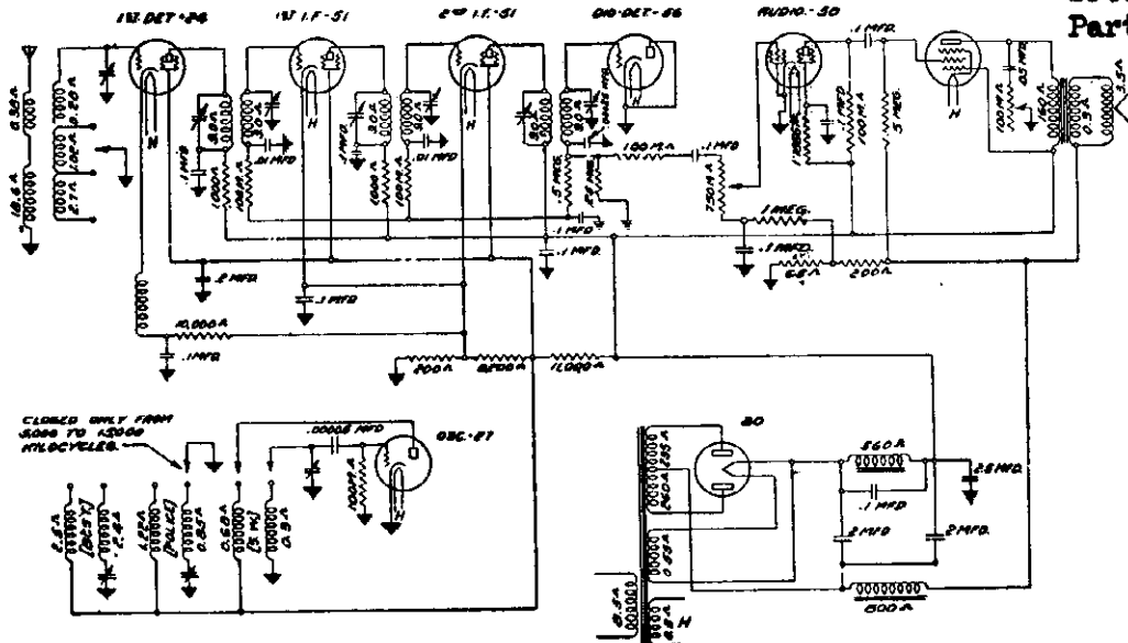
SCHEMATIC DIAGRAM OF CLARION MODEL 240 DESIGNED BY L.V. CHECKED BY [Signature] APPROVED BY [Signature] DATE: 5-17-32
