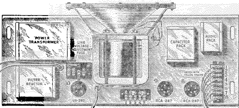
S.P.U.-REPRODUCER ASSEMBLY
