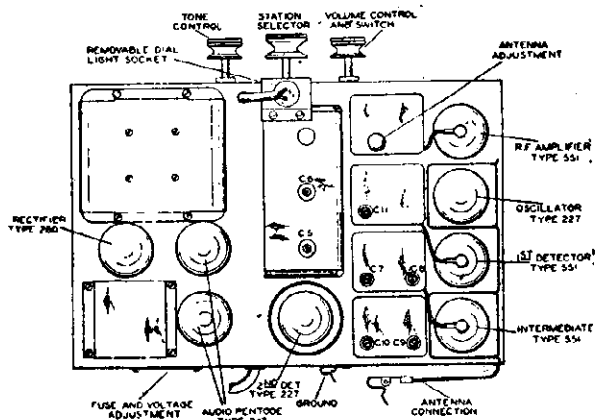
Alignment Adjustments
