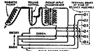
Figure 3—Magnetic Pickup connections
