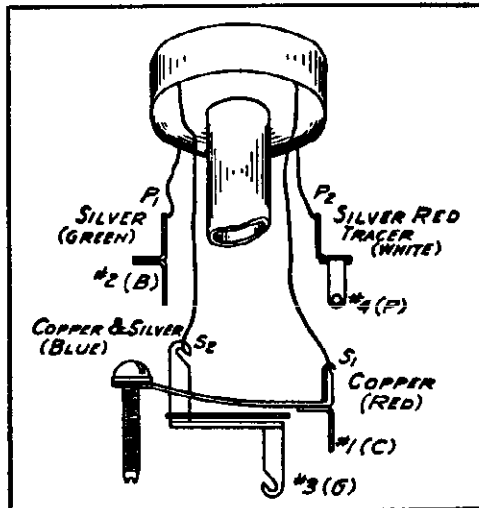
-Wiring Diagram, 2nd I.F. Assembly
