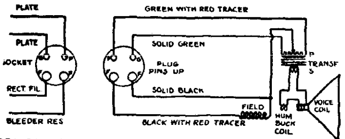
SPEAKER 287 FOR CHASSIS 123:
