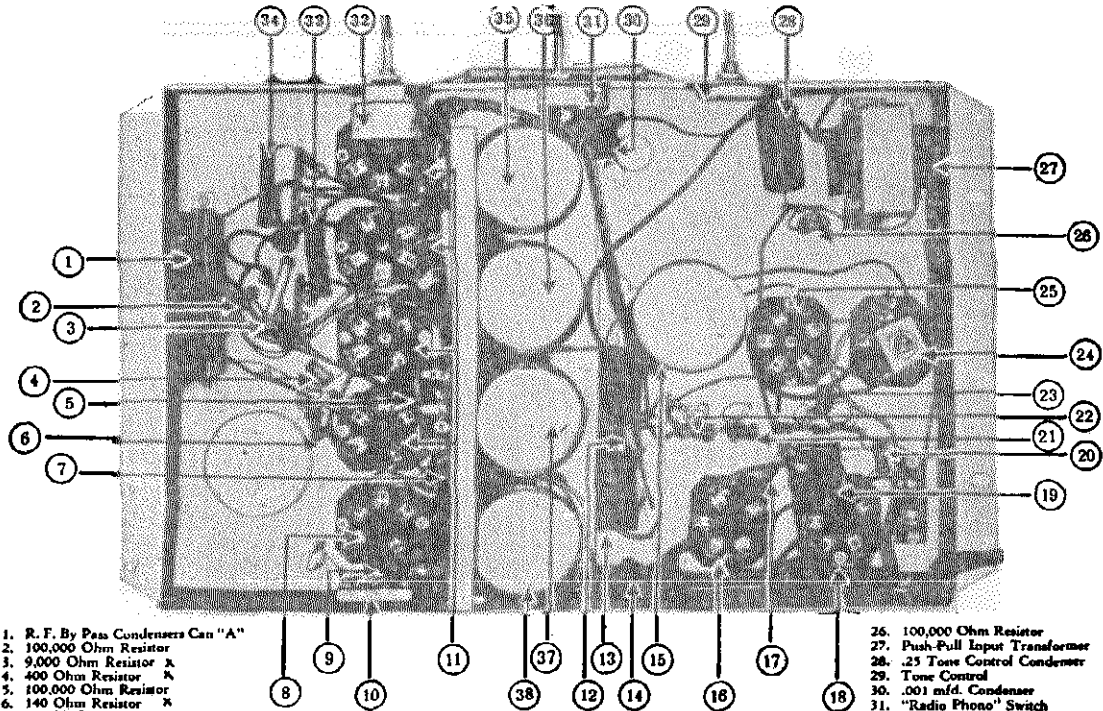
Interior View of Model 35 Chassis
