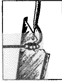
Figure 17—Proper Method of Grounding Shield When Using Plane Antenna
