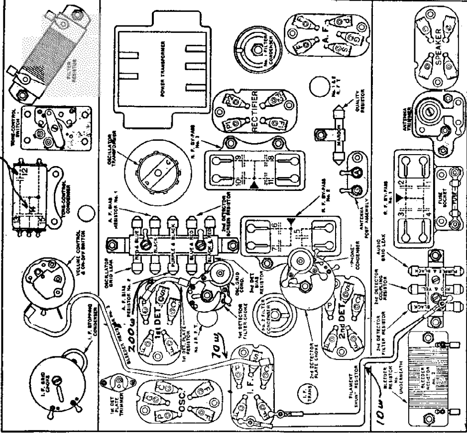
CHART OF LATE-TYPE MODEL 84, 84-F.
