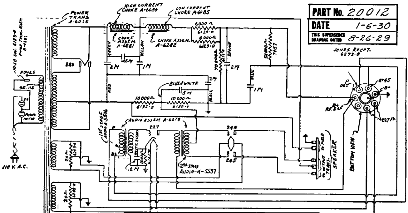
ERLA MODEL "A3" A.F. AMPLIFIER
