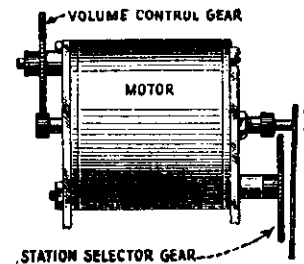
Figure 1—Motor with armature in volume control position
