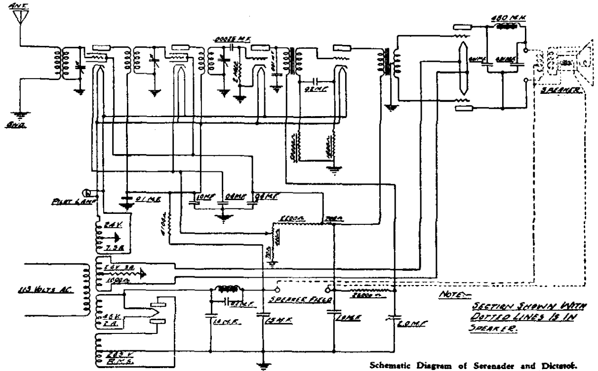
Schematic Diagram of Serenader and Dictator.
