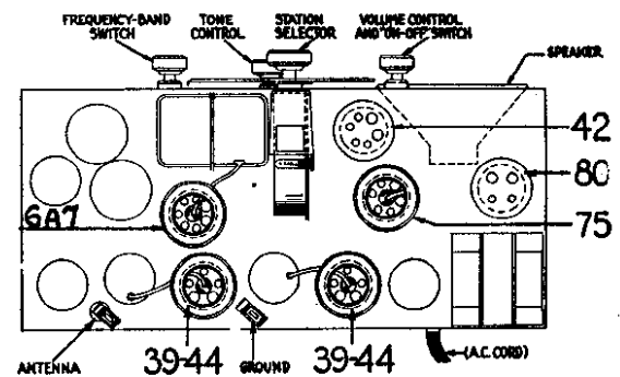
Fig. 2—Chassis Top View
