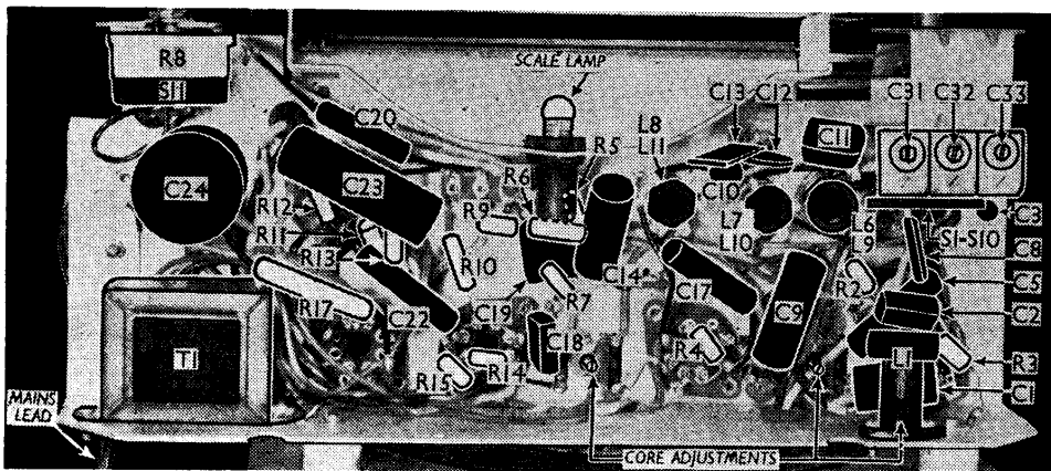
Under-chassis view. The S1-S10 switch unit, indicated here on the right, is shown in detail in a diagram inset with the circuit diagram overleaf.
