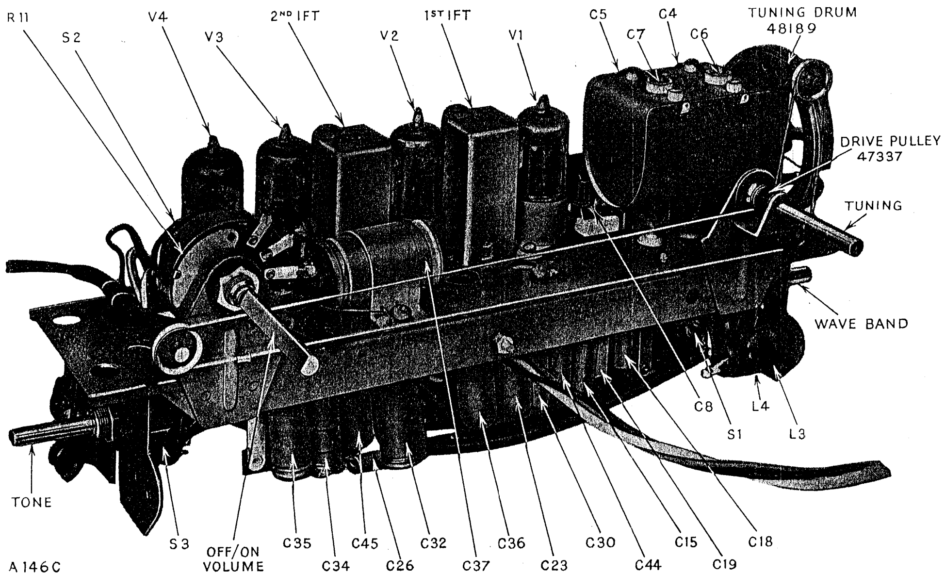
Fig. 9. Top view of the receiver chassis. The underneath view is on page 6.
