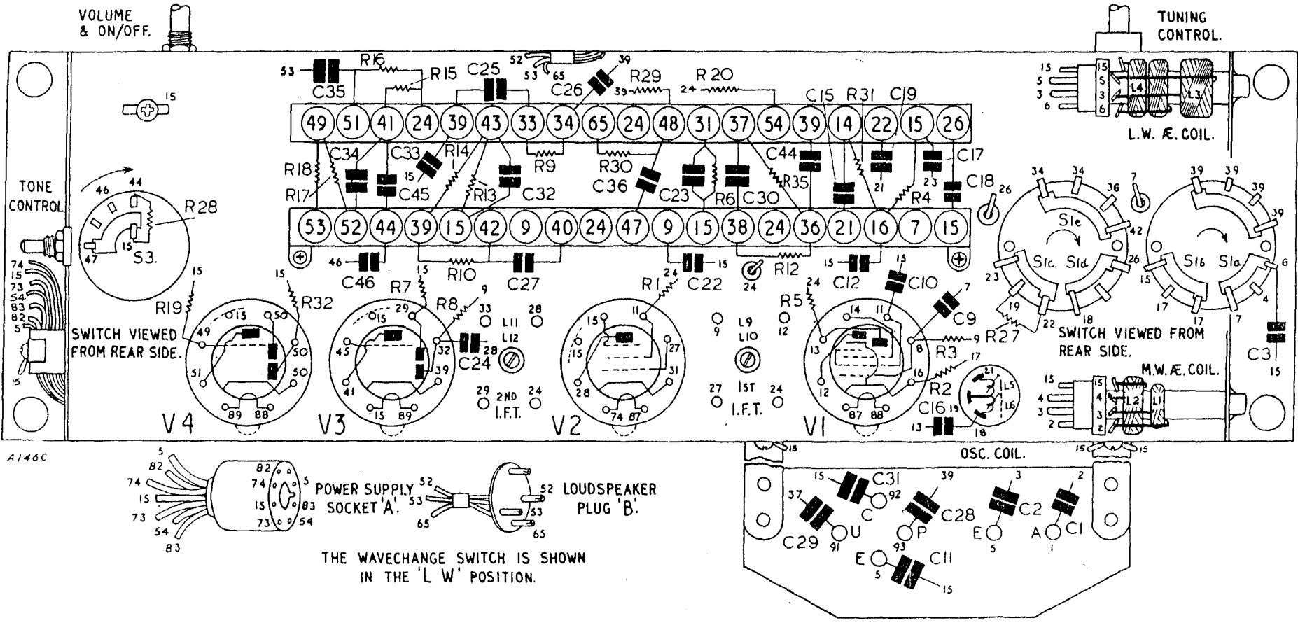
UNDERNEATH VIEW OF RECEIVER CHASSIS. Fig. 7. The diagram of the top of the receiver chassis is on page 13
