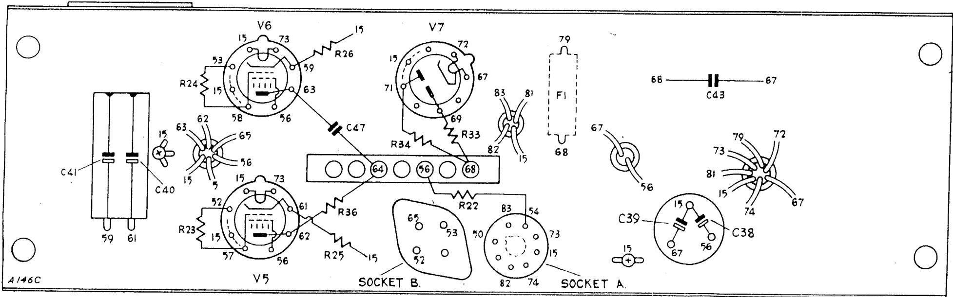
Fig. 12. Diagram of the underside of the power unit. The diagram of the top of the power unit is opposite.
