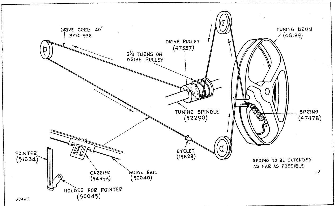
Fig. 5. The cord drive
