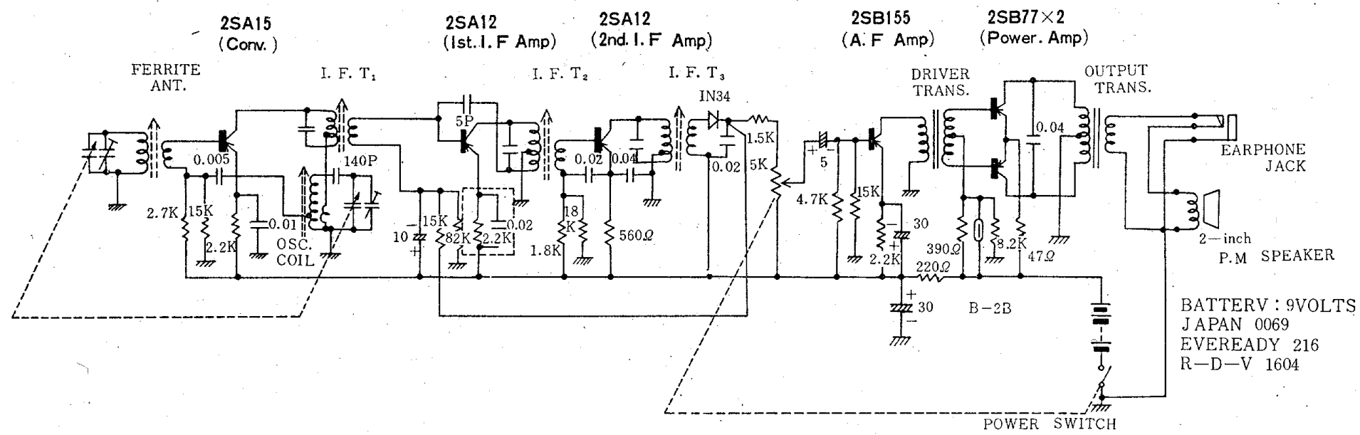
CIRCUIT DIAGRAM—HITACHI MODEL TH650
