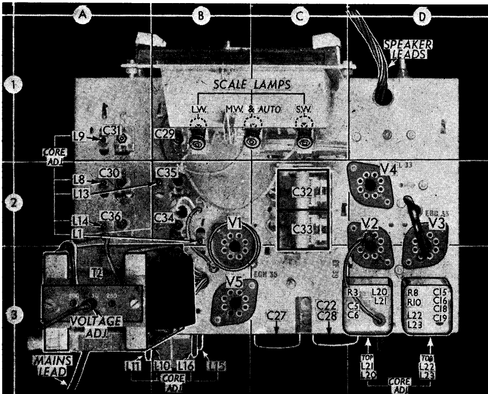
Plan view of the chassis. The four core adjustments for the pre-set tuning circuits are seen projecting from the rear. Between them is a calibrated scale to indicate the approximate wavelength.
