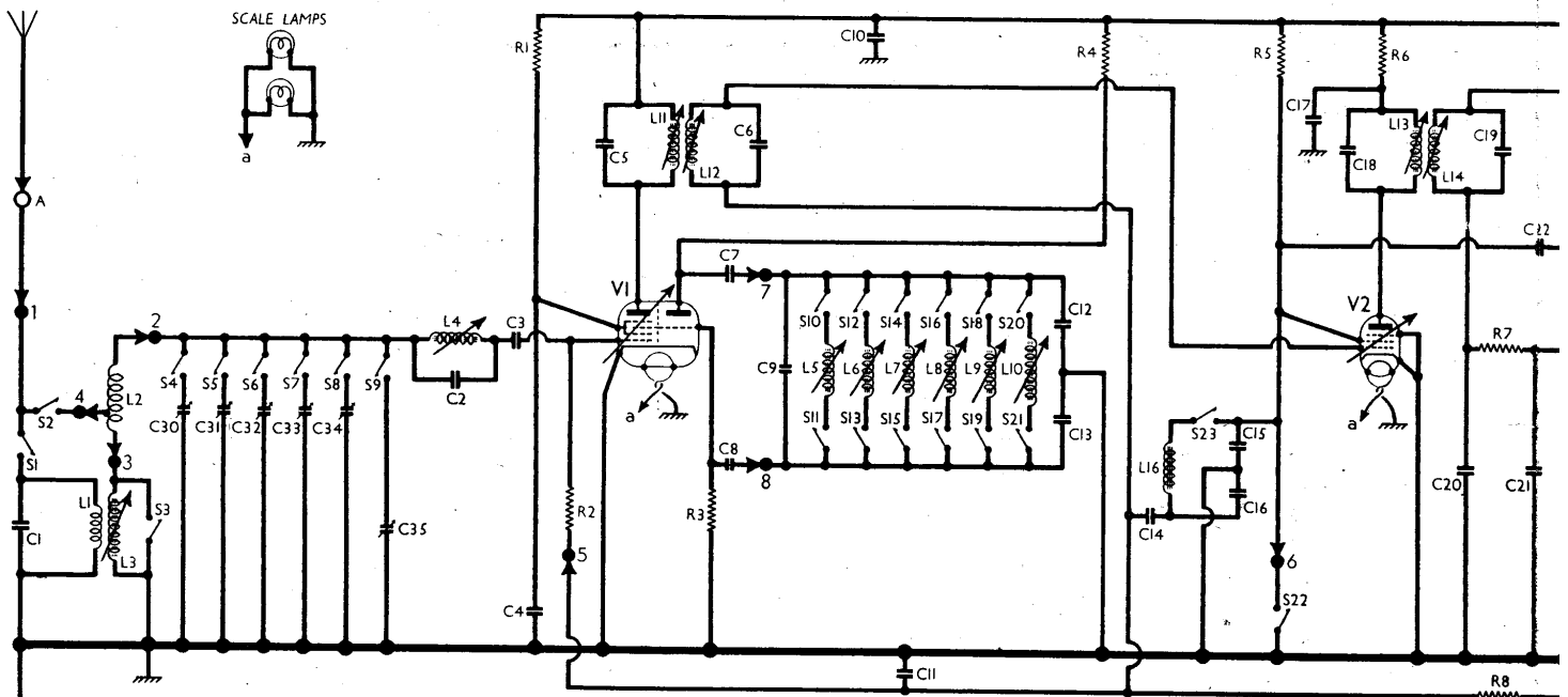
Circuit diagram of the Ekco A33 receiver. Although a frame aerial is used, provision is made for the connection of an external socket A. The numbered points in the diagram indicate the eight connections between the tuning assembly and the chassis explained in detail under "Dismantling the Set." The radio muting switch S22 closes between settings of the station selector and S23 is closed when the "Tone Alarm" facility is required. Relay winding L17 has a dual function, since it closes its associated contacts S26 , in the mains circuit, and also acts as an H.T. smoothing choke.
