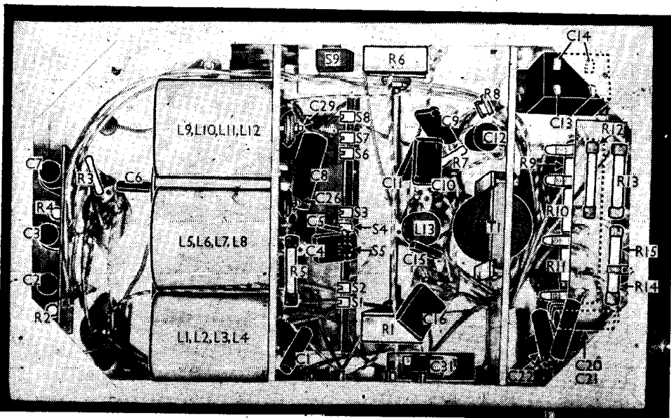
Under-chassis view. Switch numbers are shown against the spring blade tags.
