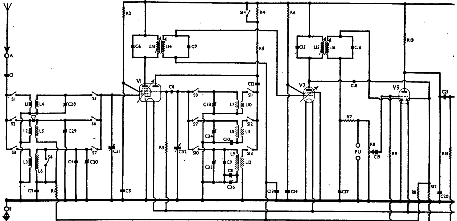
Circuit diagram of the Cossor 35 three-band battery superhet. Grid bias for all valves, and AVC delay, are automatic, and an HT circuit fuse is fitted. A similar chassis is employed in the model 37, and the differences in models 31, 32 and 439 are described under "Models 31, 32, 439." Speaker plug and valve base diagrams are inset to the right of the circuit diagram.
