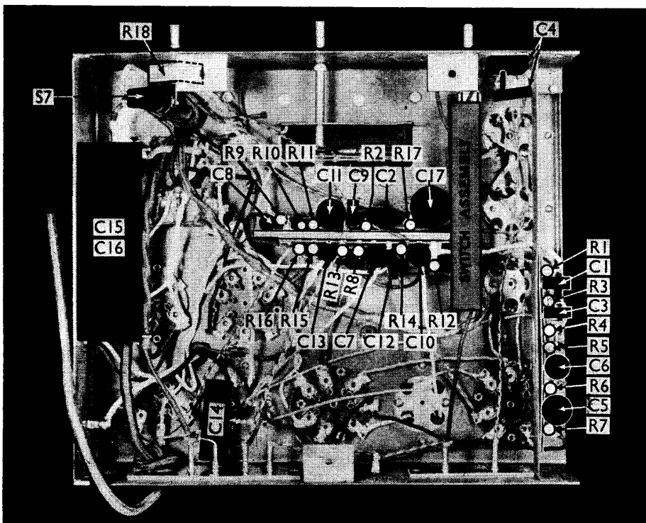
Under-chassis view. Most of the small components are seen end-on, since they are mounted on vertical paxolin strips. The switch assembly is shown in detail in the diagrams on the opposite page. Note that C4 comprises two condensers, one fixed and one pre-set. C15 and C16 are dry electrolytic condensers in one unit.
