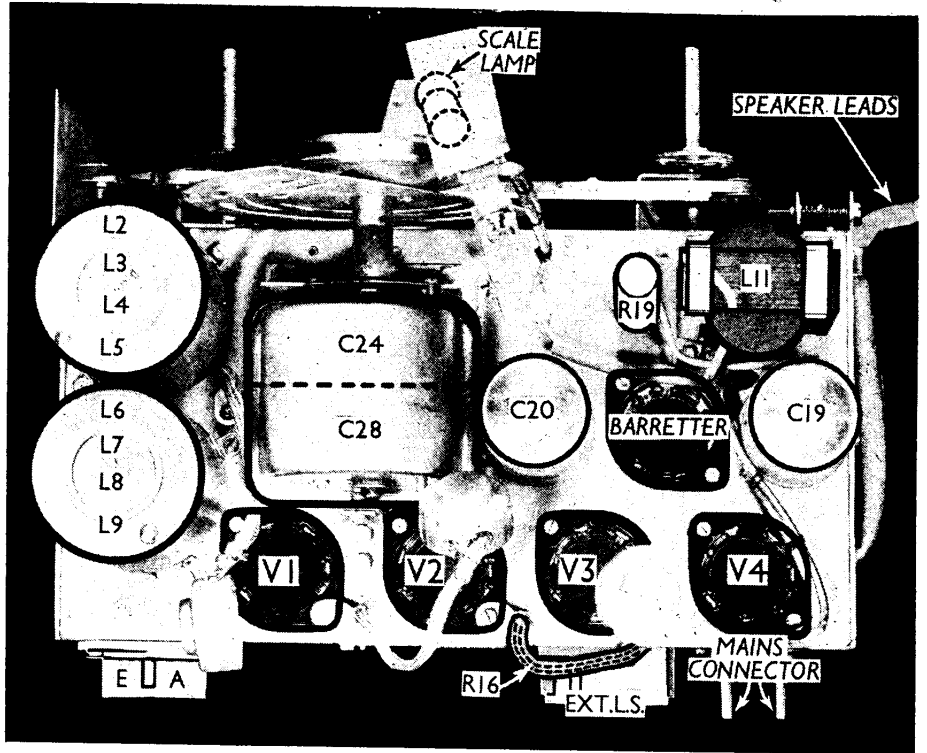
Plan view of the chassis. R16 is a flexible resistance inside the lead to the top cap of V3.
