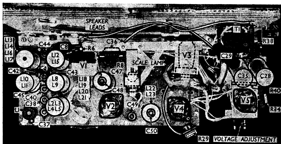
Plan view of the whole assembly, with the speaker removed. C42, C43 are wire-wound condensers.
