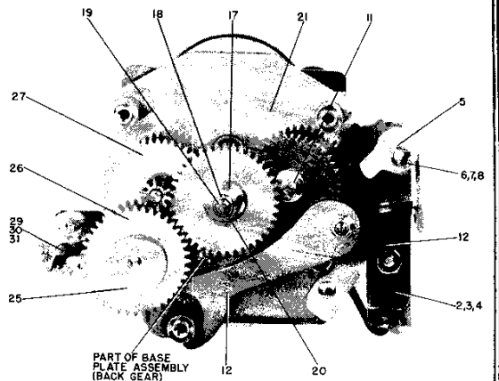
Fig. 9. Front View of C51 Clocks—Front Plate Removed
