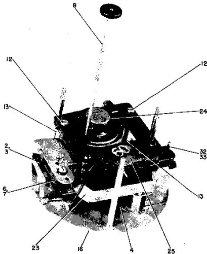
Fig. 11. Back View, C57 Clocks
