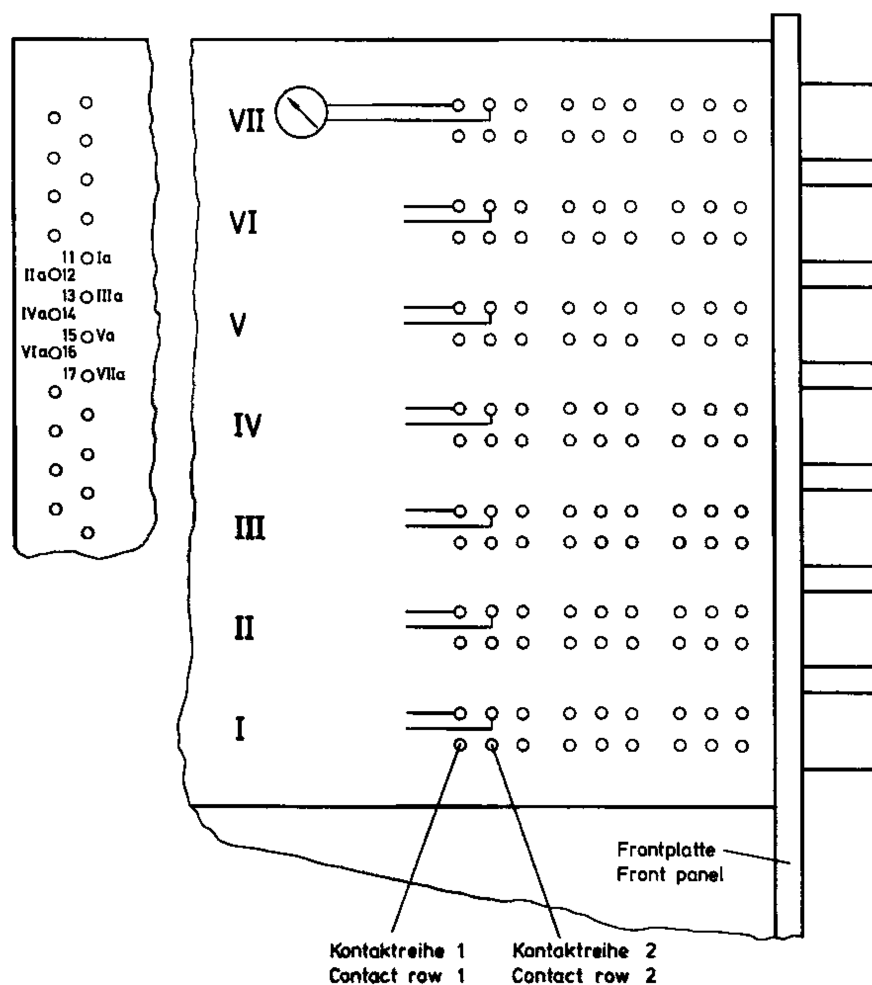
Fig. 5-2 Key set with test points
