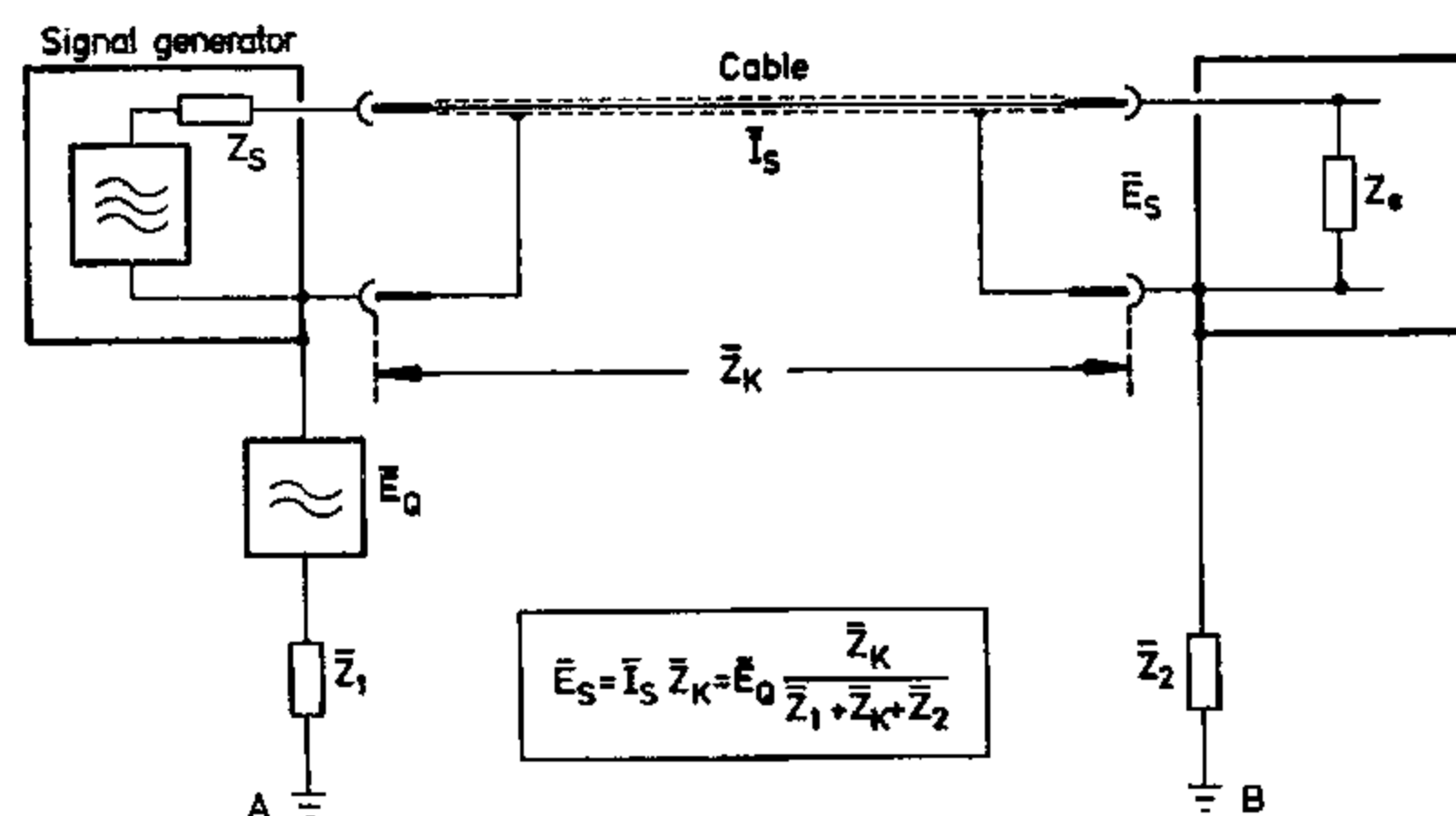
Fig. 2-4 Simplified equivalent diagram of noise voltage source
