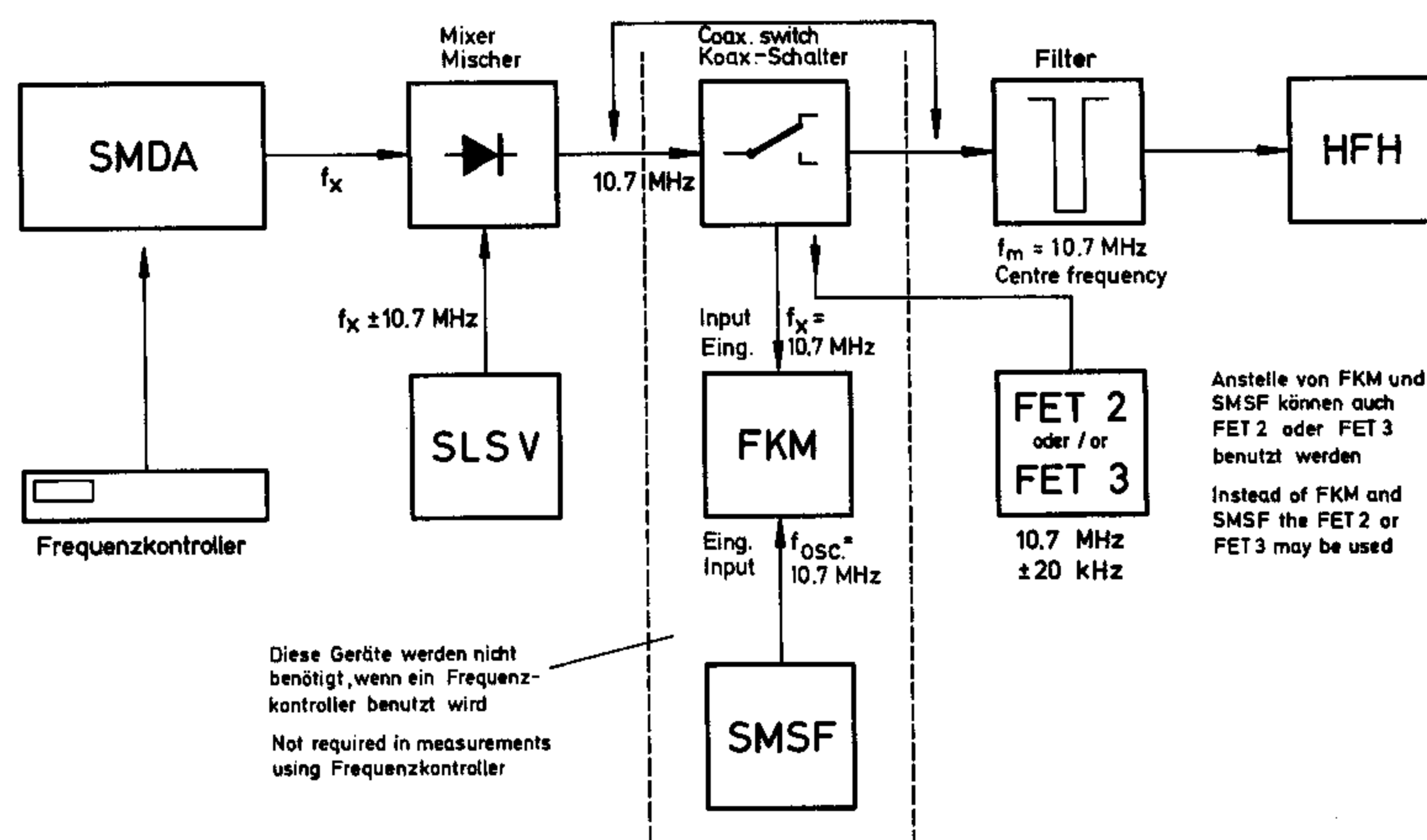
Fig. 3-6 Test setup for noise voltage measurement
