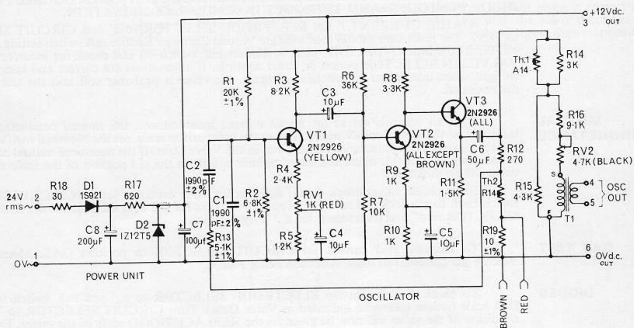
FIG. 5 OSCILLATOR AND POWER UNIT CIRCUIT DIAGRAM
