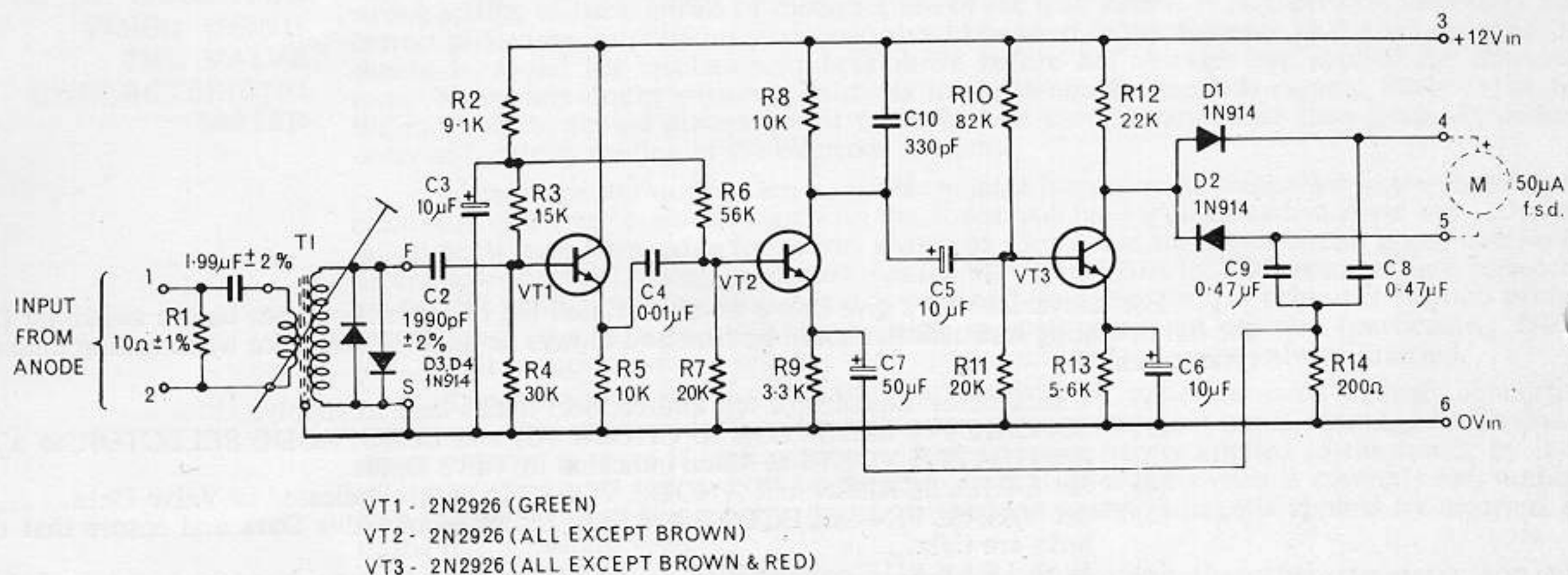
FIG. 4 AMPLIFIER CIRCUIT DIAGRAM
