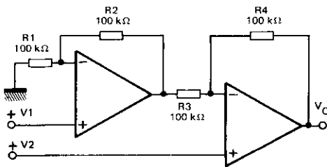
AMPLIFICATEUR DIFFERENTIEL A HAUTE IMPEDANCE D'ENTREE HIGH INPUT Z, DC DIFFERENTIAL AMPLIFIER
