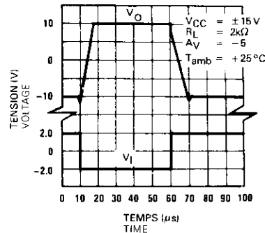
REPONSE A UNE IMPULSION DE FORTE AMPLITUDE (TDx 0149) INVERTING LARGE SIGNAL PULSE RESPONSE
