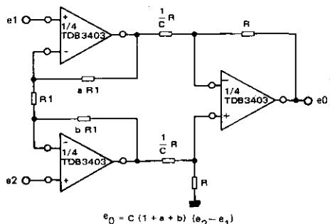
AMPLIFICATEUR DIFFERENTIEL A HAUTE IMPEDANCE HIGH IMPEDANCE DIFFERENTIAL AMPLIFIER
