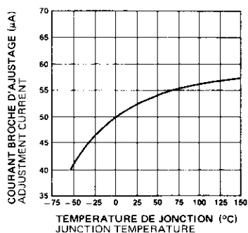
FIG. 5 — COURANT BROCHE AJUSTAGE ADJUSTMENT PIN CURRENT
