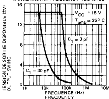
REPONSE EN FREQUENCE GRANDS SIGNAUX LARGE SIGNAL FREQUENCY RESPONSE
