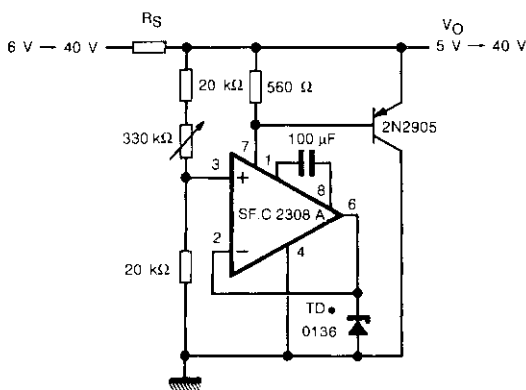
Figure 7. Régulateur shunt ajustable Adjustable shunt regulator
