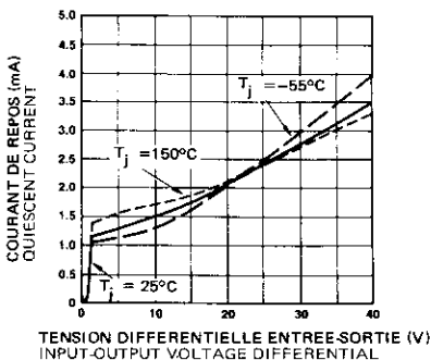
FIG. 8 — COURANT OPERATIONNEL MINIMUM MINIMUM OPERATING CURRENT
