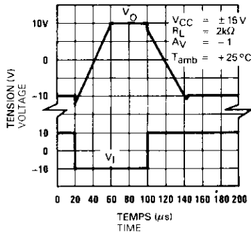
REPONSE A UNE IMPULSION DE FORTE AMPLITUDE (TDx 0148) INVERTING LARGE SIGNAL PULSE RESPONSE
