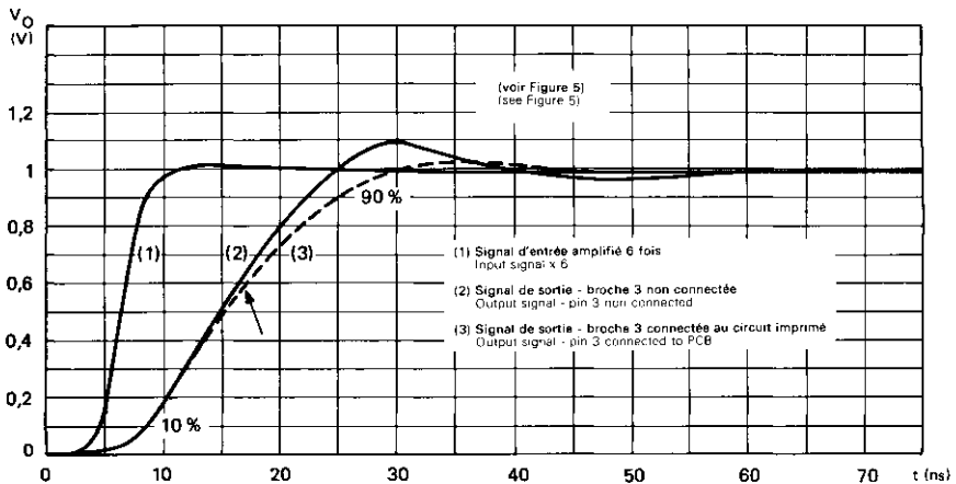
FIGURE 6: MESURE DU TEMPS DE MONTEE MEASUREMENT OF SLEW RATE
