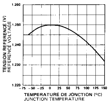
FIG. 7 — STABILITE EN TEMPERATURE TEMPERATURE STABILITY
