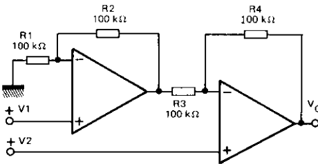
AMPLIFICATEUR DIFFERENTIEL A HAUTE IMPEDANCE D'ENTREE HIGH INPUT Z, DIFFERENTIAL AMPLIFIER
