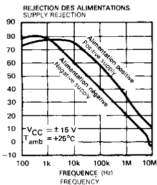
REJECTION DES ALIMENTATIONS SUPPLY VOLTAGE REJECTION RATIO
