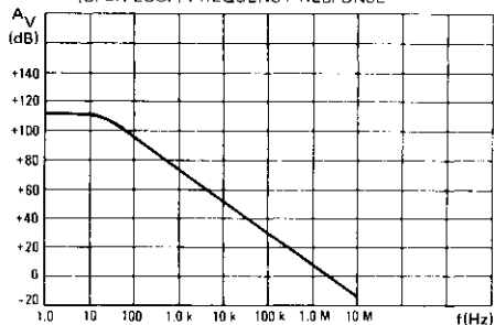
REPONSE EN FREQUENCE (BOUCLE OUVERTE) (OPEN LOOP) FREQUENCY RESPONSE
