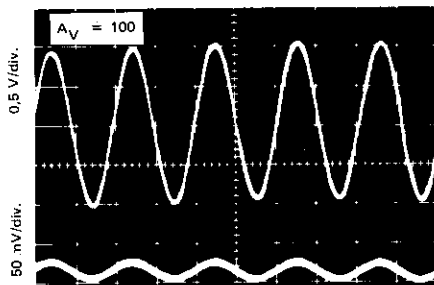
REPONSE SINUSOÏDALE SINE WAVE RESPONSE
