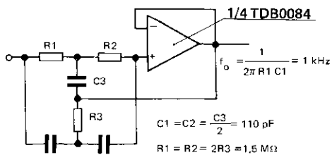
CIRCUIT BOUCHON A Q ELEVE HIGH Q NOTCH FILTER
