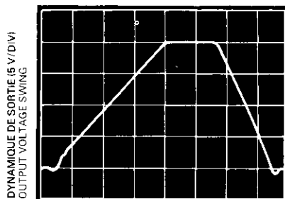
REPONSE A UNE IMPULSION DE FORTE AMPLITUDE TDC 0155 A_V = +1 LARGE SIGNAL PULSE RESPONSE
