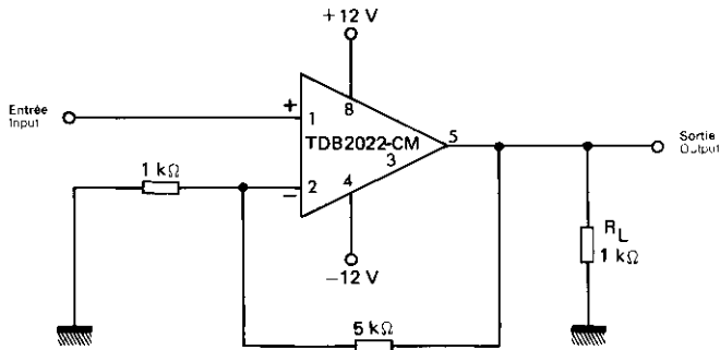
FIGURE 5: AMPLIFICATEUR NON INVERSEUR NON INVERTING AMPLIFIER A_V = +6
