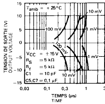
TEMPS D'ACQUISITION INVERTER SETTLING TIME
