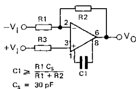
COMPENSATION A UN POLE SINGLE POLE COMPENSATION
