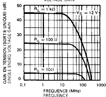
REDUCTION DU GAIN TYPIQUE TYPICAL GAIN REDUCTION
