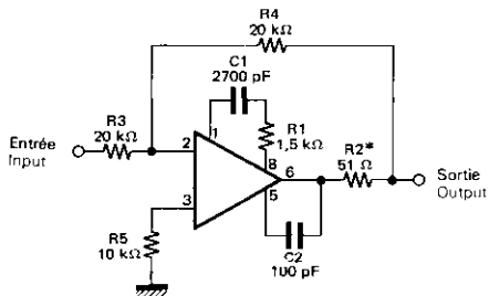
AMPLIFICATEUR INVERSEUR A GAIN UNITE UNITY GAIN INVERTING AMPLIFIER
