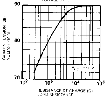
GAIN EN TENSION VOLTAGE GAIN
