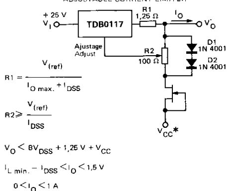
FIG.18 — LIMITATION DU COURANT AJUSTABLE ADJUSTABLE CURRENT LIMITER
