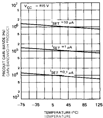
PRODUIT GAIN-BANDE GAIN BANDWIDTH PRODUCT
