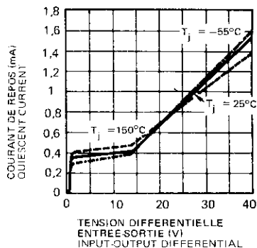
COURANT OPERATIONNEL MINIMUM MINIMUM OPERATING CURRENT
