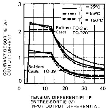
LIMITATION DE COURANT CURRENT LIMIT
