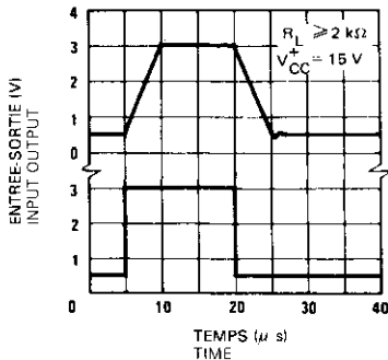
REPONSE IMPULSIONNELLE (PETITS SIGNAUX) VOLTAGE FOLLOWER PULSE RESPONSE (SMALL SIGNAL)
