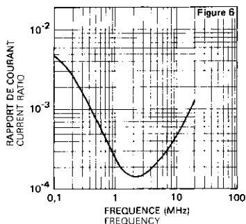
GAIN INVERSE EN COURANT ( G_{12} ) REVERSE CURRENT TRANSFER RATIO
