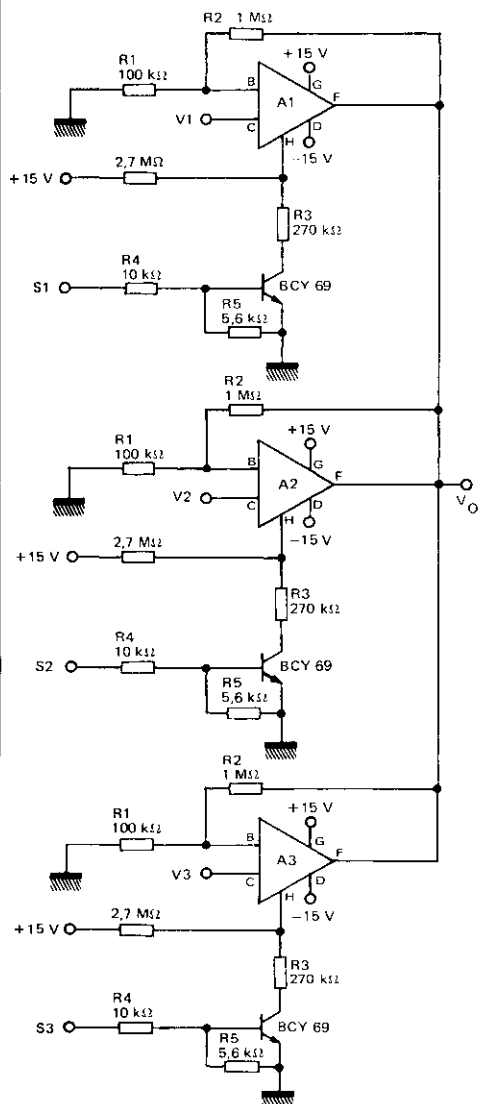
MULTIPLEXEUR SANS TRANSISTOR A EFFET DE CHAMP MULTIPLEXING AND SIGNAL CONDITION NG WITHOUT FET'S
