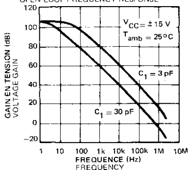
REPONSE EN FREQUENCE BOUCLE OUVERTE OPEN LOOP FREQUENCY RESPONSE
