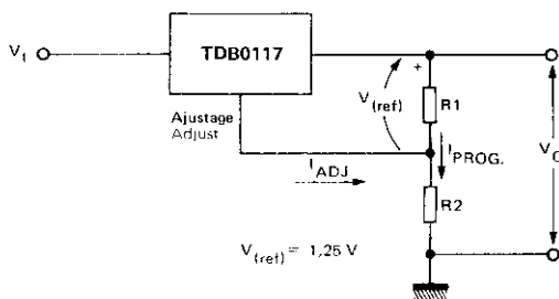
FIG.15 -- PRINCIPE DE BROCHAGE BASIC CIRCUIT CONFIGURATION
