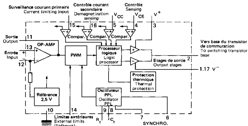
SCHEMA - BLOC BLOCK DIAGRAM
