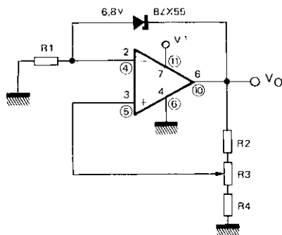
TENSION DE REFERENCE POSITIVE POSITIVE VOLTAGE REFERENCE
