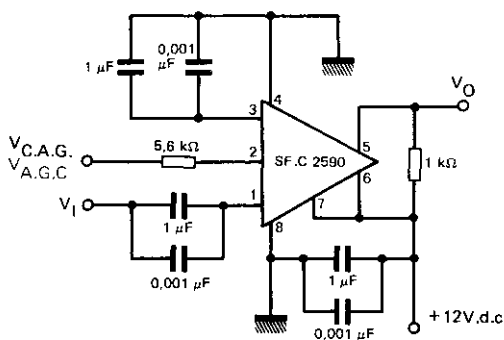
FIGURE 3 AMPLIFICATEUR 30 MHz ( G_p = 50 dB, B \approx 1 MHz) 30 MHz AMPLIFIER
