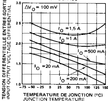
FIG. 6 — TENSION DIFFERENTIELLE ENTREE-SORTIE DROPOUT VOLTAGE
