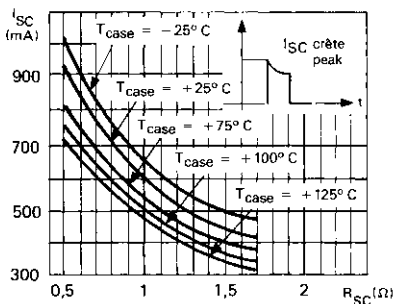
AIRE DE FONCTIONNEMENT DE SECURITE (SURCHARGE NON REPETITIVE) SAFE OPERATING AREA (NON REPETITIVE OVER LOAD)
