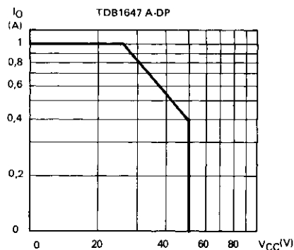
SAIE DE FONCTIONNEMENT DE SECURITE (SURCHARGE NON REPETITIVE) SAFE OPERATING AREA (SURGE NON REPETITIVE)
