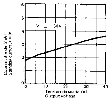
COURANT A VIDE STANDBY CURRENT DRAIN
