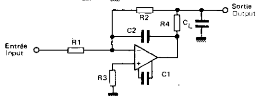
ISOLEMENT DES CHARGES TRES CAPACITIVES ISOLATING LARGE CAPACITIVE LOADS
