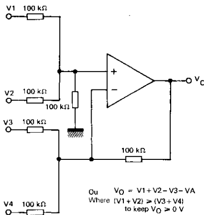
AMPLIFICATEUR NON-INVERSEUR, TENSION CONTINUE NON-INVERTING AMPLIFIER, DC
