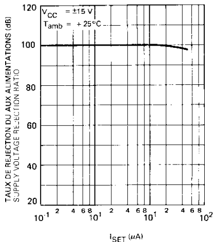
TAUX DE REJECTION DU AUX ALIMENTATIONS SUPPLY VOLTAGE REJECTION RATIO
