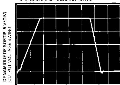
REPONSE A UNE IMPULSION DE FORTE AMPLITUDE TDC 0156 A_V = +1 LARGE SIGNAL PULSE RESPONSE
