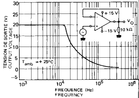
BANDE PASSANTE POWER BANDWIDTH
