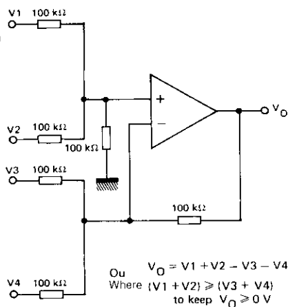
AMPLIFICATEUR NON-INVERSEUR, TENSION CONTINUE NON-INVERTING DC GAIN
