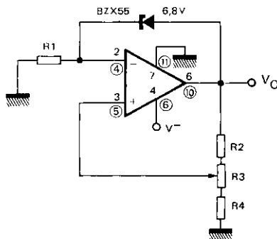
TENSION DE REFERENCE NEGATIVE NEGATIVE VOLTAGE REFERENCE
