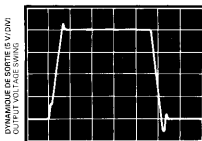
REPONSE A UNE IMPULSION DE FORTE AMPLITUDE TDC 0157 A_V = +5 LARGE SIGNAL PULSE RESPONSE
