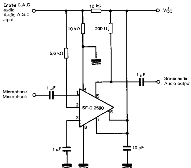
FIGURE 6 COMPRESSEUR DE PAROLE SPEECH COMPRESSOR
