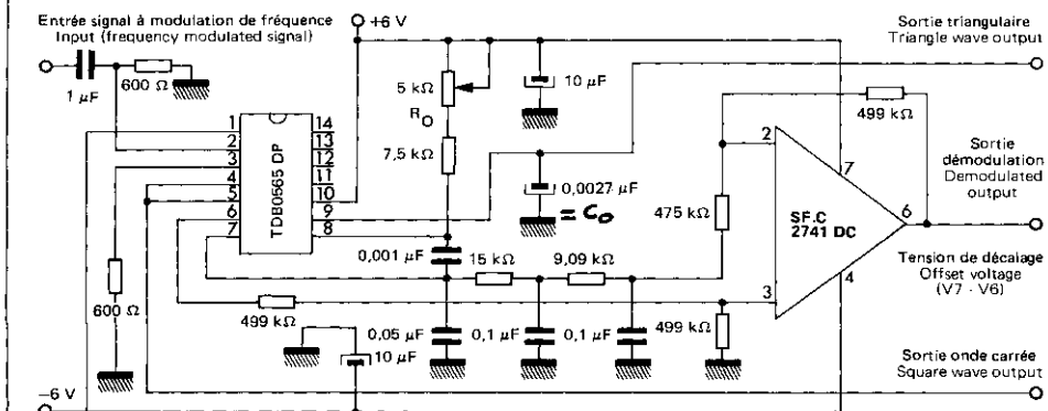
FIGURE 2 — SCHEMA DU CIRCUIT DE TEST TEST CIRCUIT SCHEMATIC
