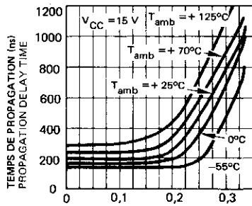
TENSION MINIMALE DE L'IMPULSION DE DECLENCHEMENT ( \times V_{CC} ) LOWEST VOLTAGE LEVEL OF TRIGGER PULSE
