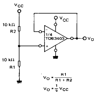
REFERENCE DE TENSION VOLTAGE REFERENCE
