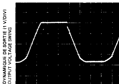
LIMITATION DE COURANT ( R_L = 100 \Omega ) CURRENT LIMIT
