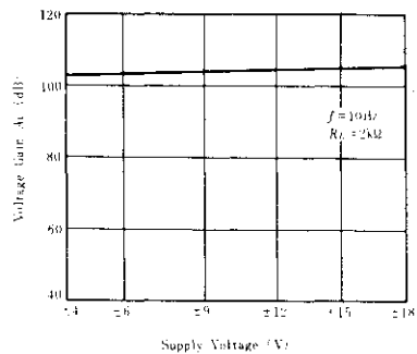
VOLTAGE GAIN VS. SUPPLY VOLTAGE
