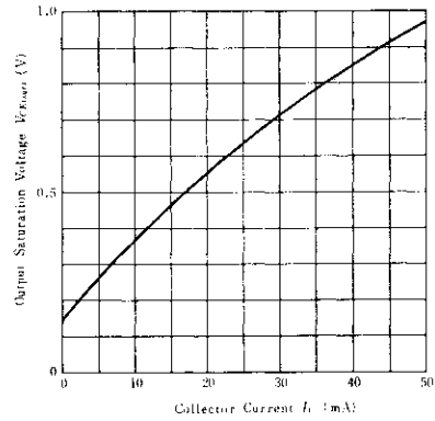
OUTPUT SATURATION VOLTAGE VS. COLLECTOR CURRENT
