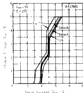
(c) Output Voltage vs Input Voltage
