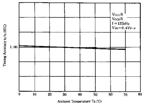
TIMING ACCURACY VS. AMBIENT TEMPERATURE
