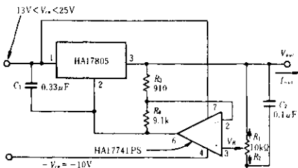
Fig.17 Variable Output Voltage (0.5 to 10V) Regulator
