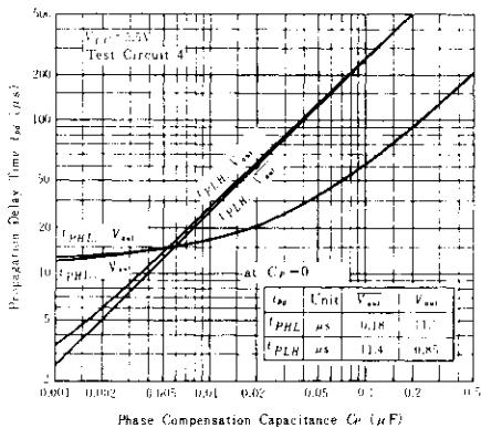
PROPAGATION DELAY TIME VS. PHASE COMPENSATION CAPACITANCE
