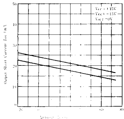
OUTPUT SHORT CURRENT VS. AMBIENT TEMPERATURE
