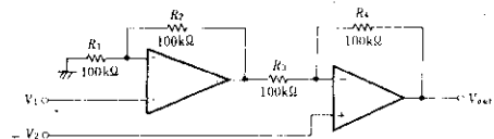
Fig.3 High Input Impedance DC Differential Amplifier
