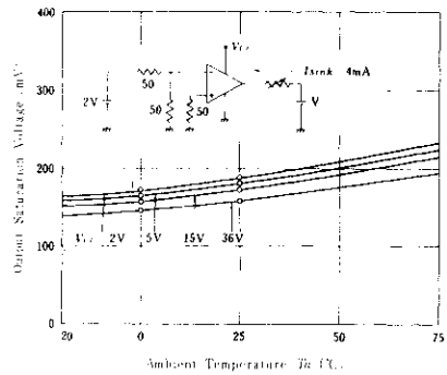
OUTPUT SATURATION VOLTAGE VS. AMBIENT TEMPERATURE
