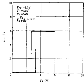
Fig.4(a) Operation Waveform of Schmitt Trigger Circuit ( V_{out} - V_s )
