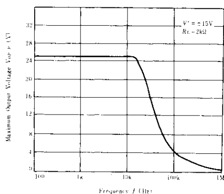
MAXIMUM OUTPUT VOLTAGE VS. FREQUENCY
