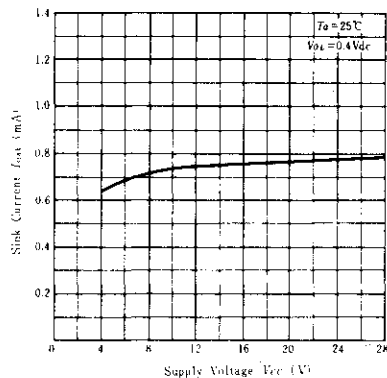
SINK CURRENT VS. SUPPLY VOLTAGE
