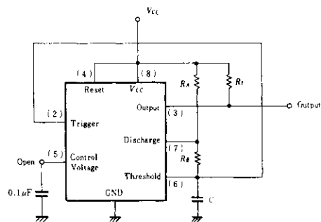
Fig.4 Astable Circuit
