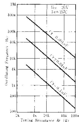
Fig. 3 Oscillating Frequency vs Timing Resistance
