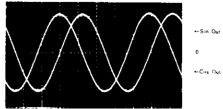
axis of ordinates 5V/DIV quadrature axis 0.2ms/DIV circuit constant C 71 = 1000pF (990) C 72 = 1000pF (990) R 71 = 150kΩ R 72 = 150kΩ C 1 = 1000pF (990) R 1 = 160kΩ R 11 = 15kΩ R 22 = 10kΩ R 33 = 16V R 44 = 10kΩ V CC = 15V V EE = -15V
