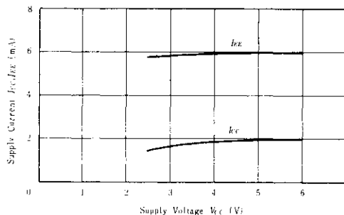
SUPPLY CURRENT VS. SUPPLY VOLTAGE (2)
