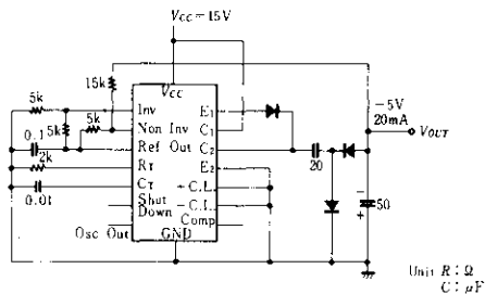
Fig.10 Simple Type Polarity Conversion
