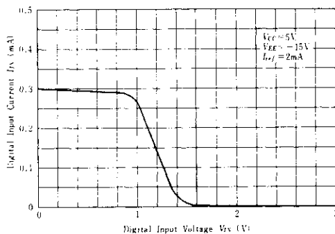
DIGITAL INPUT CURRENT VS. DIGITAL INPUT VOLTAGE
