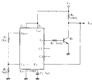
Fig.6 Fixed Voltage Source in Parallel Control
