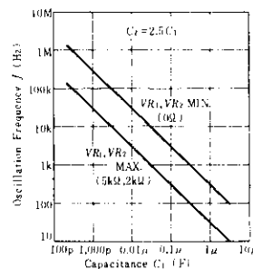
Fig.9 Oscillation Frequency vs Capacitance
