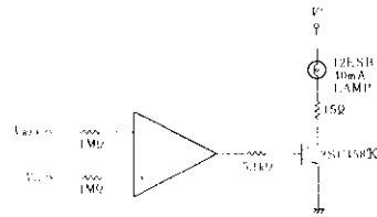
Fig.13 Power Comparator
