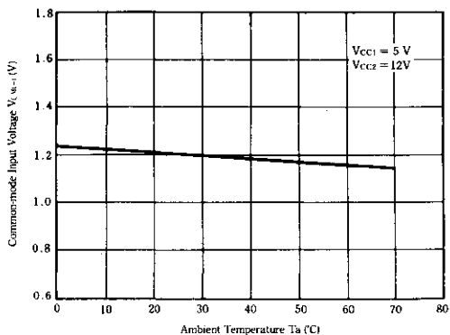
COMMON-MODE INPUT VOLTAGE VS. AMBIENT TEMPERATURE
