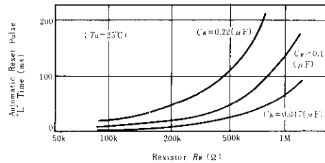
Fig. 4 R_L -Reset "L" Time Characteristics
