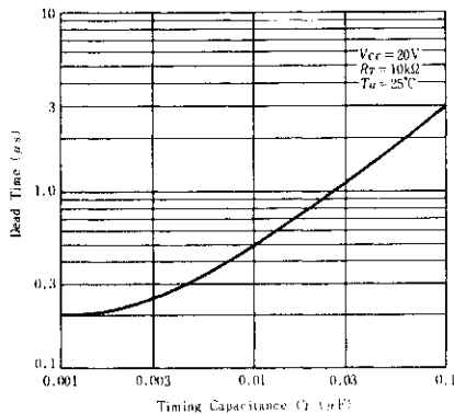
DEAD TIME VS. TIMING CAPACITANCE
