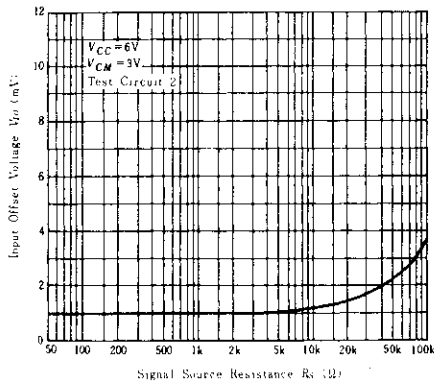
INPUT OFFSET VOLTAGE VS. SIGNAL SOURCE RESISTANCE
