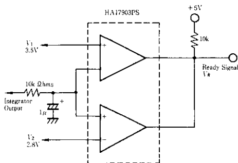
Fig. 5 Producing the Ready Signal
