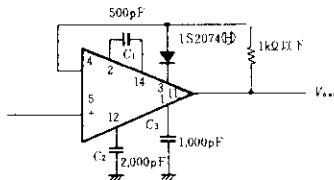
Fig.1 Phase Compensation in case voltage gain is 1
