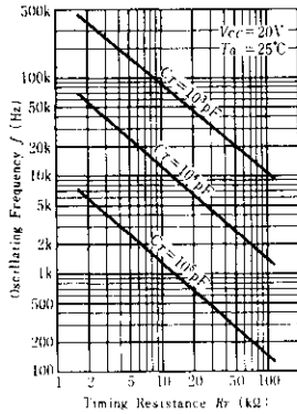
OSCILLATING FREQUENCY VS. TIMING RESISTANCE
