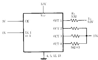
Fig. 2 Output Short Test
