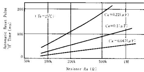
Fig. 3 R_L -Reset "H" Time Characteristics
