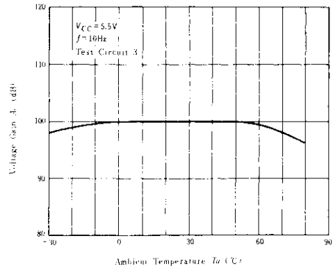
VOLTAGE GAIN VS. AMBIENT TEMPERATURE
