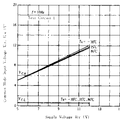
COMMON MODE INPUT VOLTAGE VS. SUPPLY VOLTAGE
