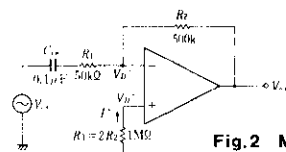
Fig.2 Mono Power Source Biasing Method
