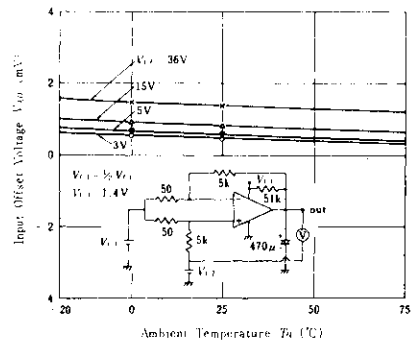
INPUT OFFSET VOLTAGE VS. AMBIENT TEMPERATURE
