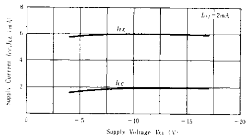
SUPPLY CURRENT VS. SUPPLY VOLTAGE (2)
