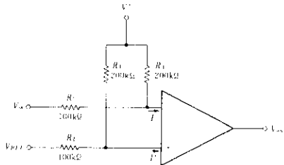
Fig.10 Negative Input Voltage Comparator
