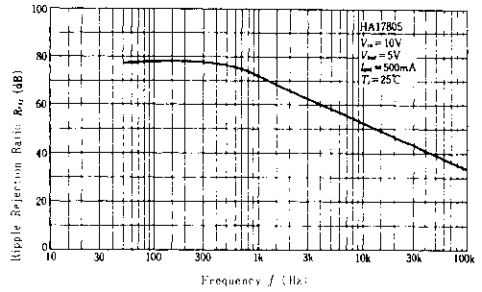
RIPPLE REJECTION VS. FREQUENCY RATIO
