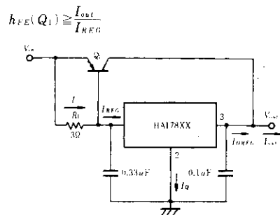
Fig.19 Regulator with Increased Output Current (1)
