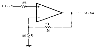
Fig.1 Non-inverted Amplifier
