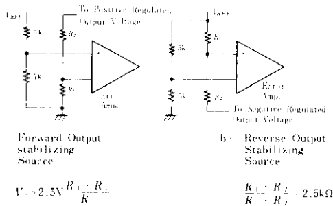
Fig. 2 Biasing in Error-Amplifier
