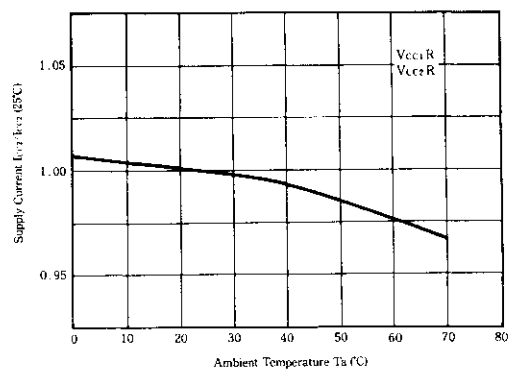
SUPPLY CURRENT VS. AMBIENT TEMPERATURE (2)
