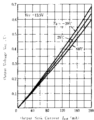
OUTPUT VOLTAGE VS. OUTPUT SINK CURRENT
