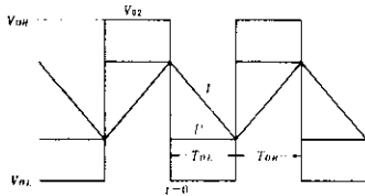
Fig.5 Operation of Triangular Wave Generator
