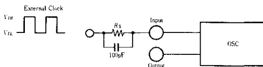
Fig. 4 Providing External Clock
