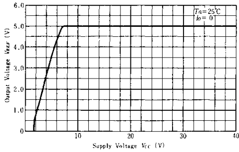
OUTPUT VOLTAGE VS. SUPPLY VOLTAGE
