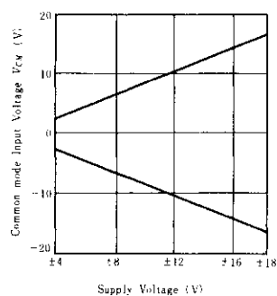
COMMON-MODE INPUT VOLTAGE VS. SUPPLY VOLTAGE
