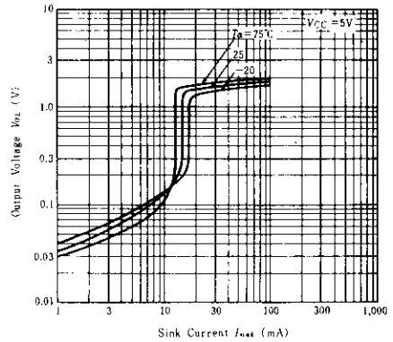
OUTPUT VOLTAGE (V&lt;sub&gt;OL&lt;/sub&gt;) VS. SINK CURRENT (I)
