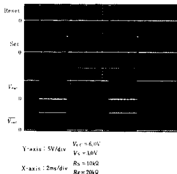
Fig.8 Operation Waveform of Bistable Circuit
