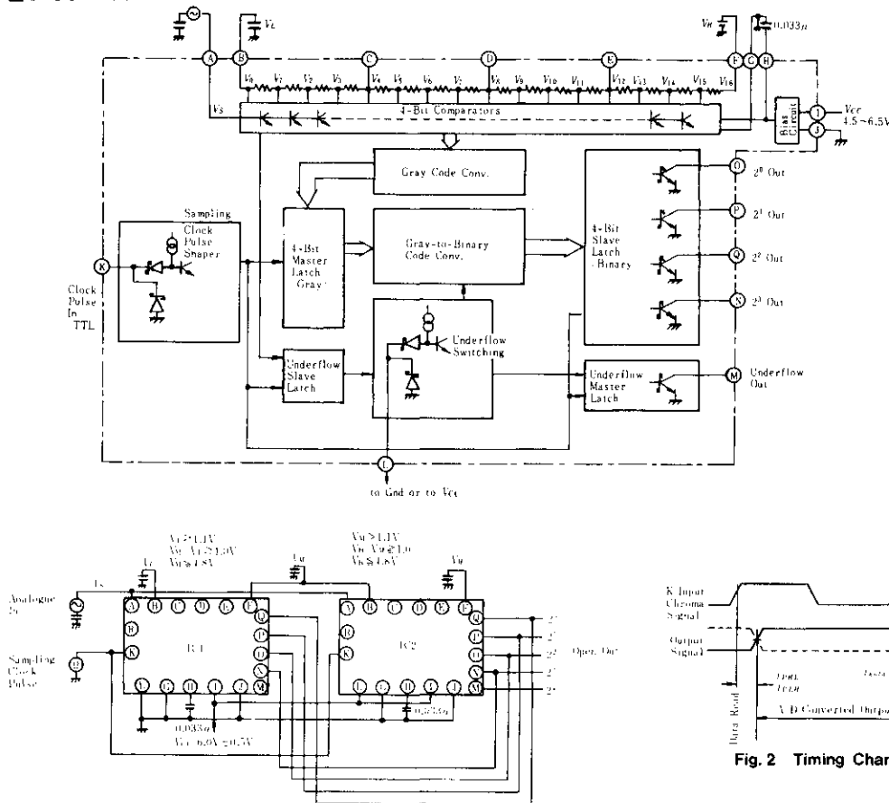
Fig. 1 Expansion to 5-bit A/D Converter
