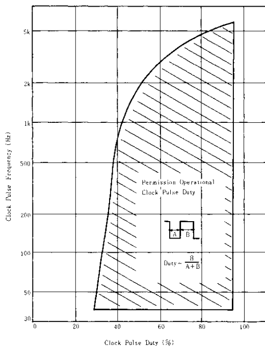
Fig. 6 Permission Operational Clock Pulse Duty VS. Frequency
