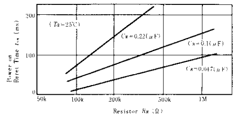
Fig. 5 R_L -ton Characteristics
