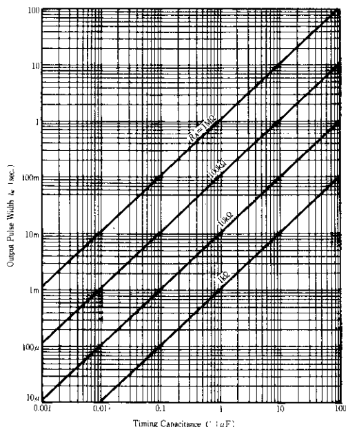
Fig.2 Output Pulse Width vs. Timing Capacitance
