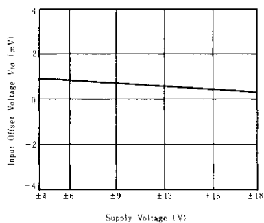
INPUT OFFSET VOLTAGE VS. SUPPLY VOLTAGE
