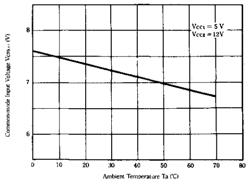
COMMON-MODE INPUT VOLTAGE VS. AMBIENT TEMPERATURE
