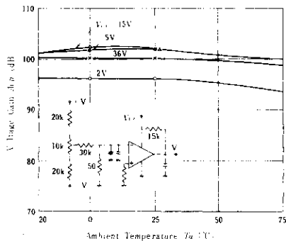
VOLTAGE GAIN VS. AMBIENT TEMPERATURE
