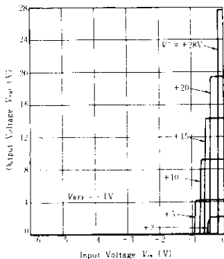
Fig.11 Operation Characteristics of Negative Input Comparator (1)
