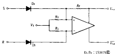
Fig.7 Bistable Circuit
