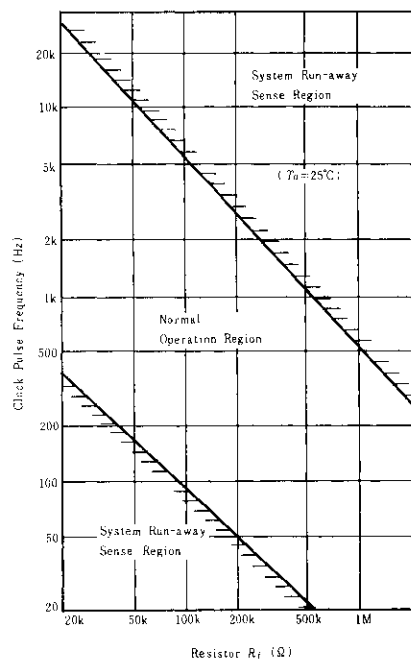
Fig. 7 Clock Pulse Frequency Input Range VS. R_1
