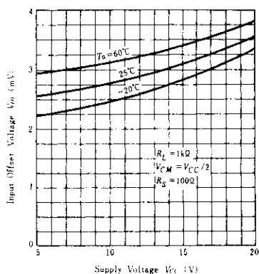
INPUT OFFSET VOLTAGE VS. SUPPLY VOLTAGE
