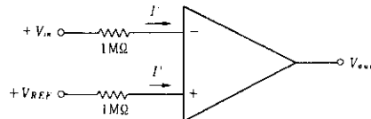
Fig.7 Positive Input Voltage Comparator
