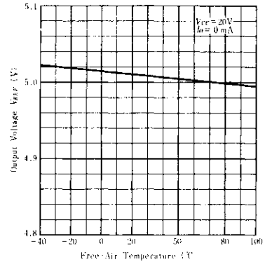
OUTPUT VOLTAGE VS. FREE AIR TEMPERATURE
