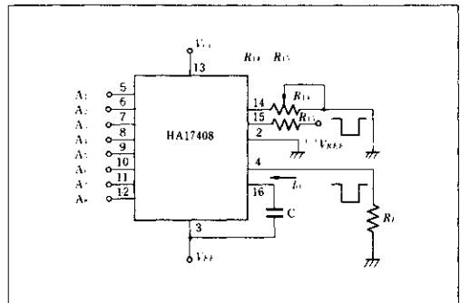
Fig. 2 Negative Reference Voltage
