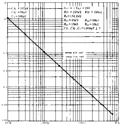
Fig.11 HA17747 Quadrature Sine Wave Oscillator f-C 71 , C 72 , C 1 characteristic
