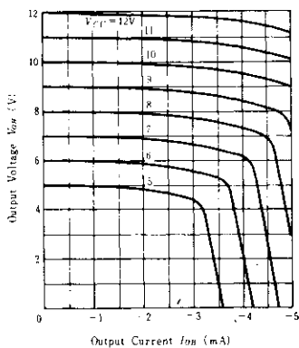
OUTPUT VOLTAGE VS. OUTPUT CURRENT
