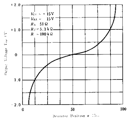
HA17083 OFFSET ADJUSTING
