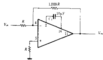
Fig.4 Phase Compensation in case voltage gain is 1000
