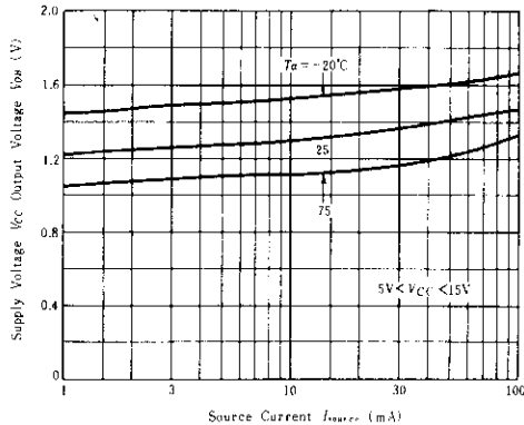
SUPPLY VOLTAGE (V&lt;sub&gt;CC&lt;/sub&gt;)-OUTPUT VOLTAGE (V&lt;sub&gt;OH&lt;/sub&gt;) VS. SOURCE CURRENT
