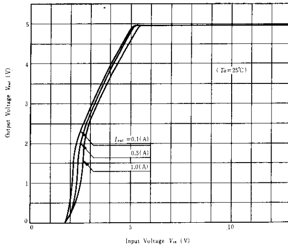
Fig. 1 Vin-Vout Characteristics
