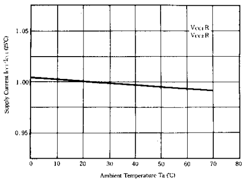
SUPPLY CURRENT VS. AMBIENT TEMPERATURE (1)
