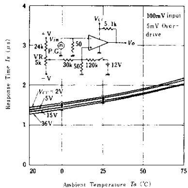
RESPONSE TIME VS. AMBIENT TEMPERATURE
