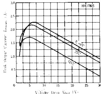
(b) Peak Output Current vs Voltage Drop
