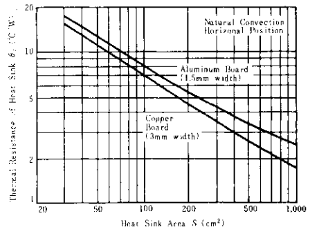
Fig.4 Areas vs Thermal Resistance of Heat Sink
