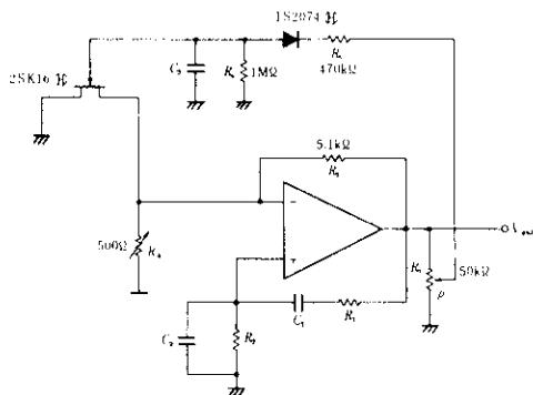
Fig.7 Wien bridge sine wave oscillator
