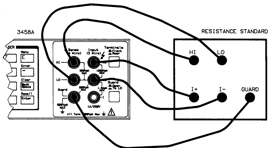
Figure 3. Resistance and DC Current Adjustment Connections
