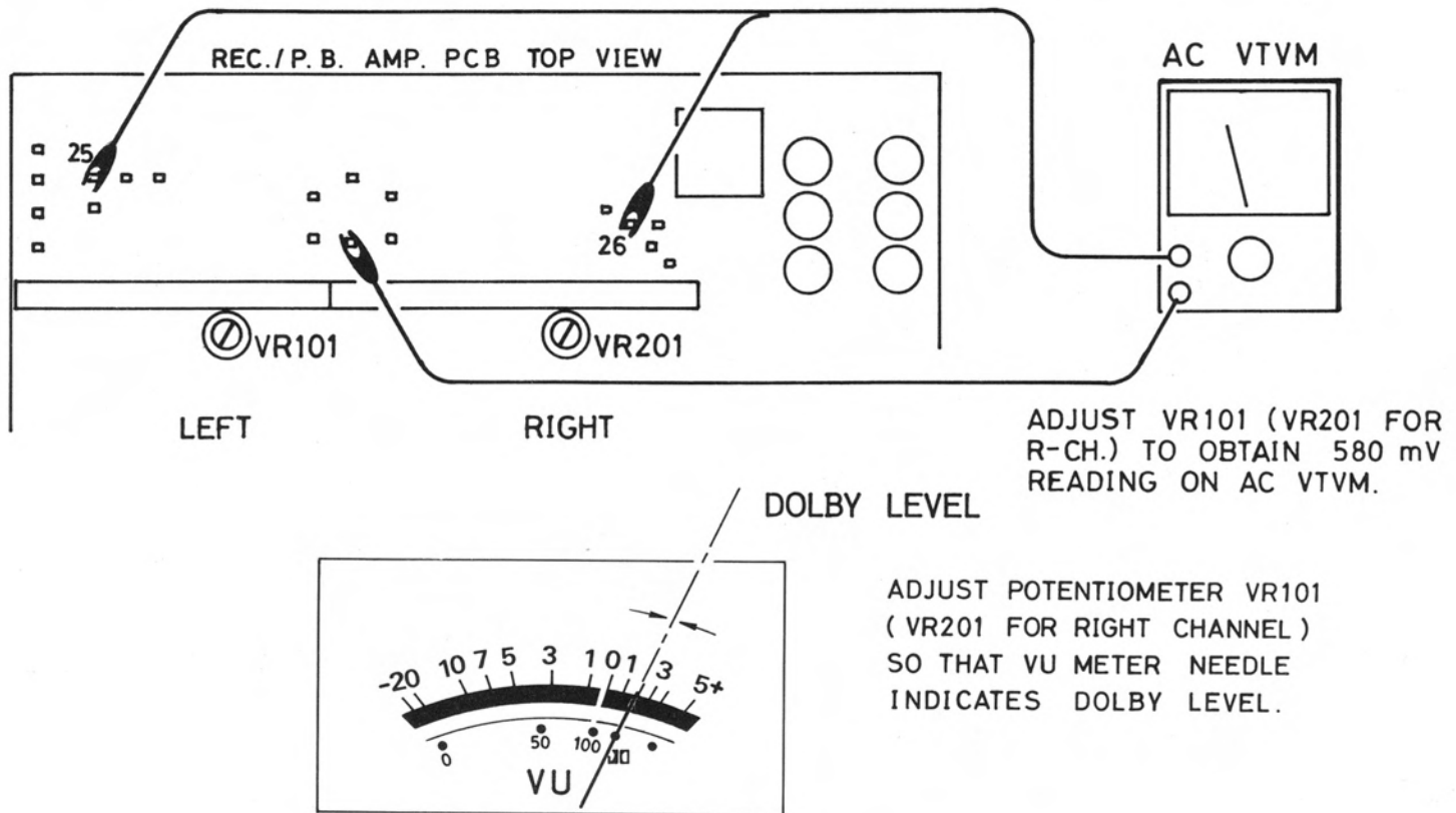
FIG. 1 DOLBY LEVEL ADJUSTMENT HOOK-UP
