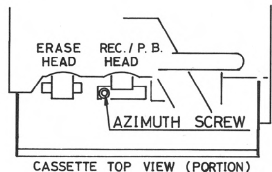
FIG. 2 AZIMUTH ADJUSTMENT
