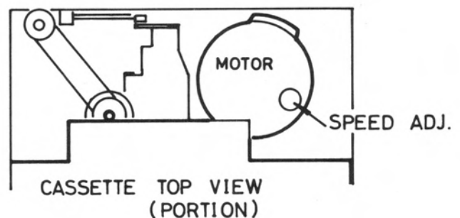
FIG. 9 TAPE SPEED ADJUSTMENT
