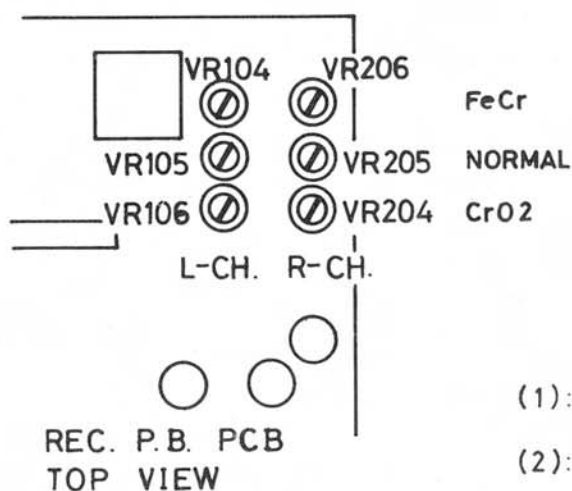
FIG. 7 BIAS CURRENT ADJUSTMENT HOOK-UP
