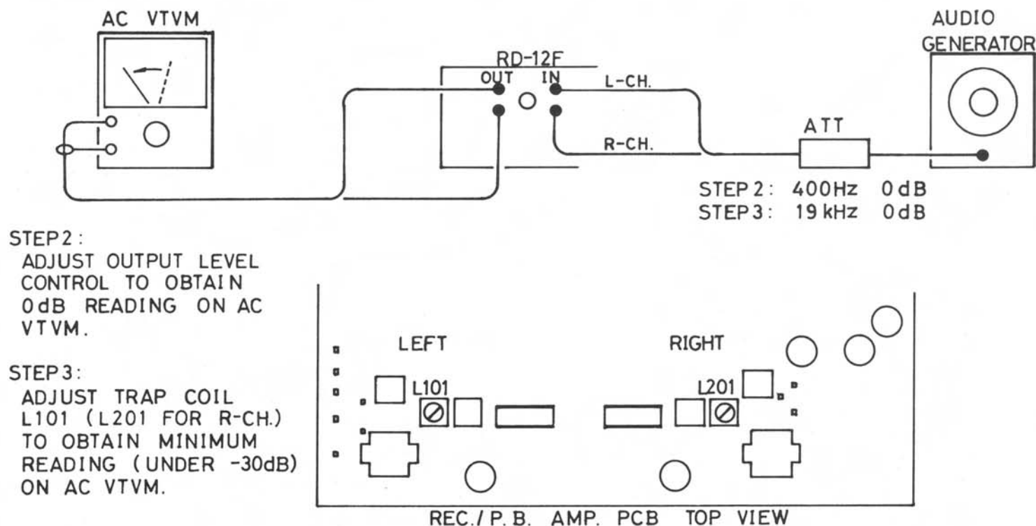
FIG. 3 19kHz TRAP COIL ADJUSTMENT HOOK-UP
