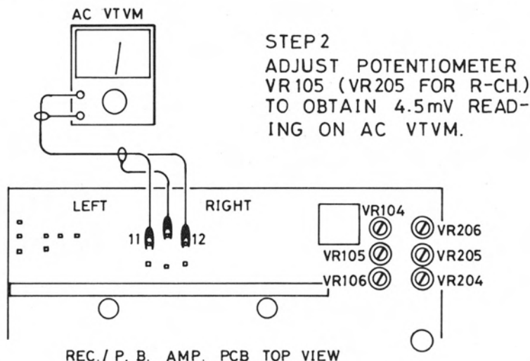
FIG. 5 BIAS VOLTAGE LEVEL ADJUSTMENT HOOK-UP
