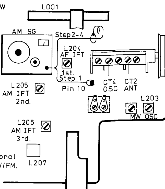
Fig. 2. AM IF and RF Alignment Hook-Up (RT-726)
