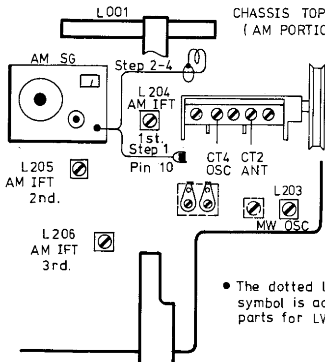
Fig. 1. AM IF and RF Alignment Hook-Up (RT-426)
