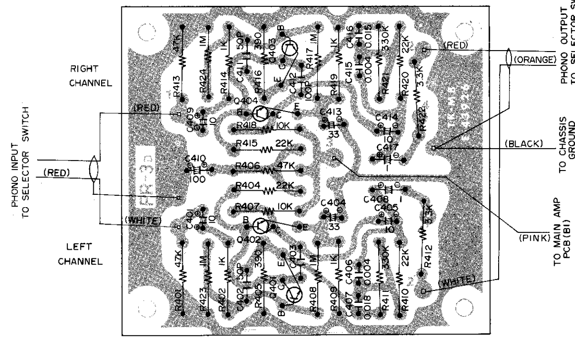
EQUALIZER AMPLIFIER CIRCUIT BOARD DIAGRAM
