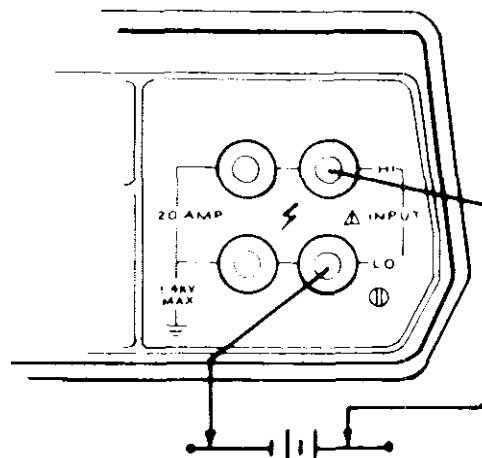
Figure 2-3. DC Voltage Measurement
