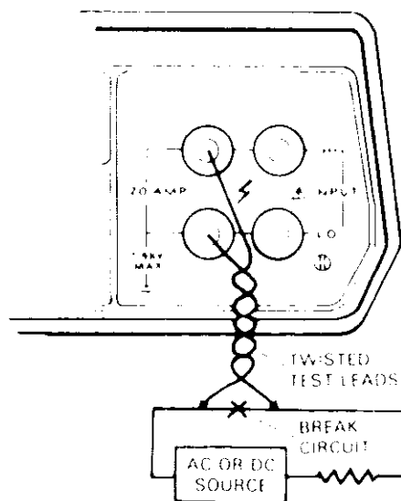
Figure 2-7. Current Measurements Between 2000mA and 20A
