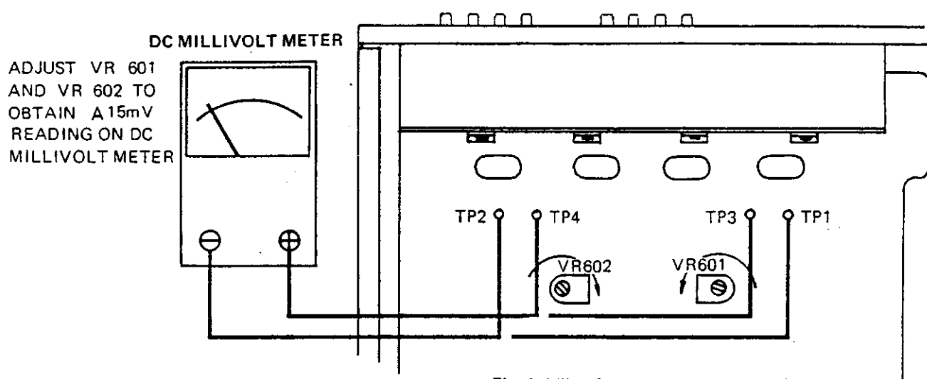
Fig. 1. Idling Current Adjustment Hook-up
