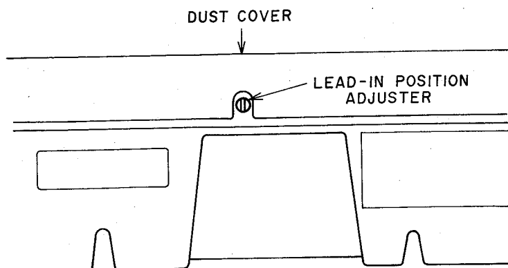
Fig. 6-2 Rear View
