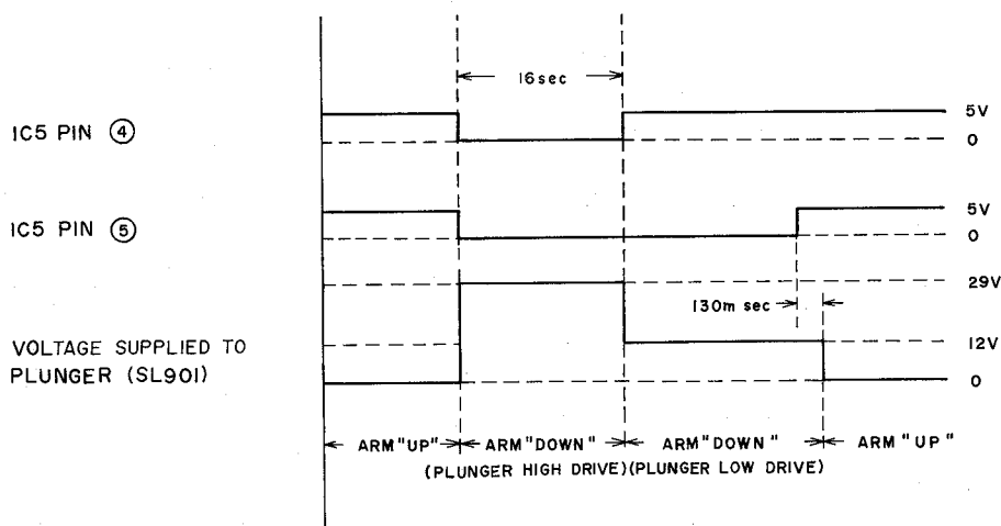
Fig. 5-7 Timing Chart
