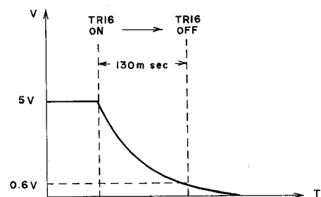
Fig. 5-6 Voltage at the Collector of TR16
