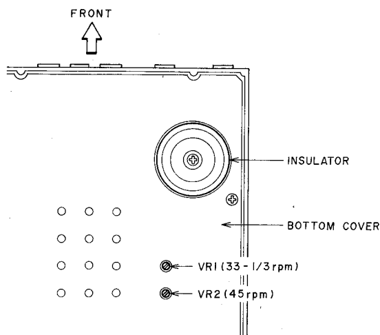
Fig. 7-2 Bottom View
