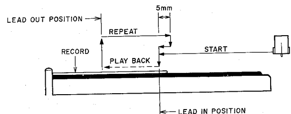
Fig. 5-3 17 cm Record
