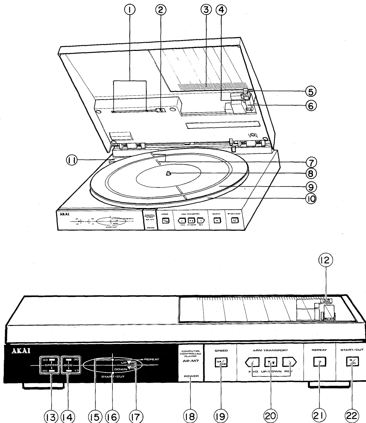
Fig. 3-1 Controls
