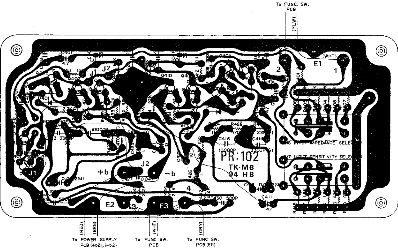
PHONO AMP. CIRCUIT BOARD DIAGRAM
