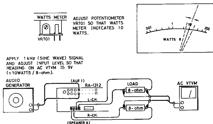
Fig.2 WATTS METER CALIBRATION HOOK-UP
