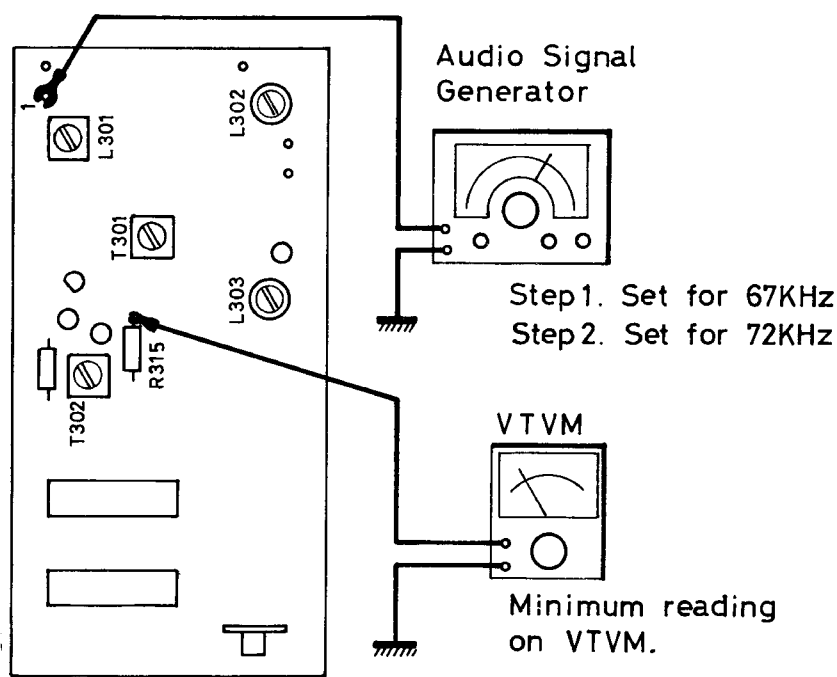
Fig2. FM-Stereo SCA Trap Adjustment Hook-up
