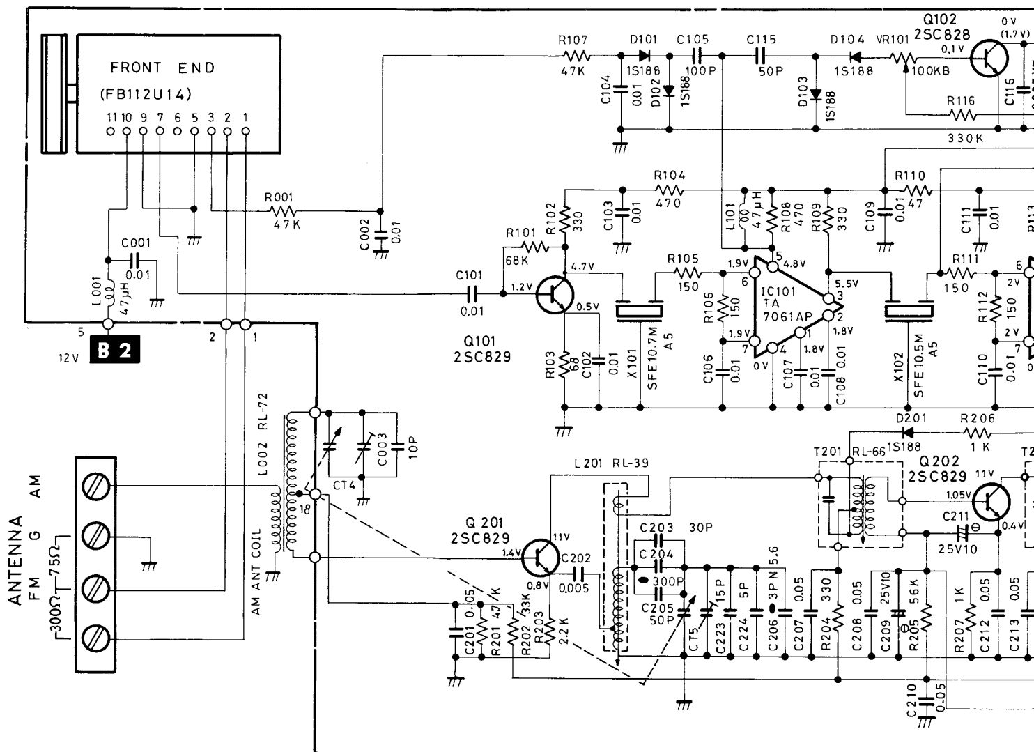
CERAMIC FILTER
