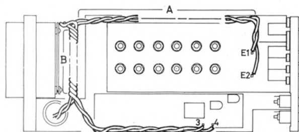
Fig. 7 WIRING DIAGRAM OF OUTPUT CIRCUIT
