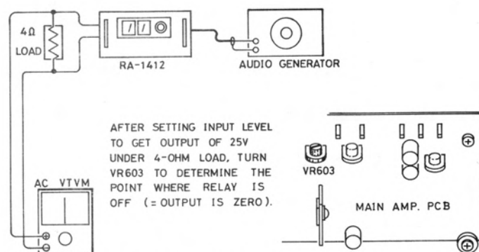
Fig. 4 OVERLOAD PROTECTION LEVEL ADJUSTMENT HOOK-UP
