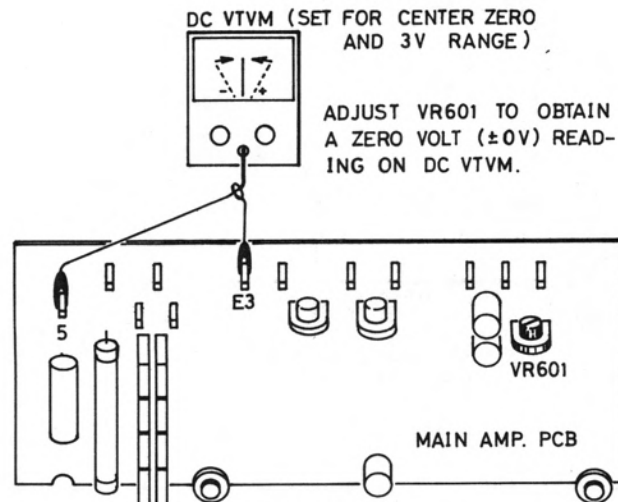
Fig.2 DC BALANCE ADJUSTMENT HOOK-UP
