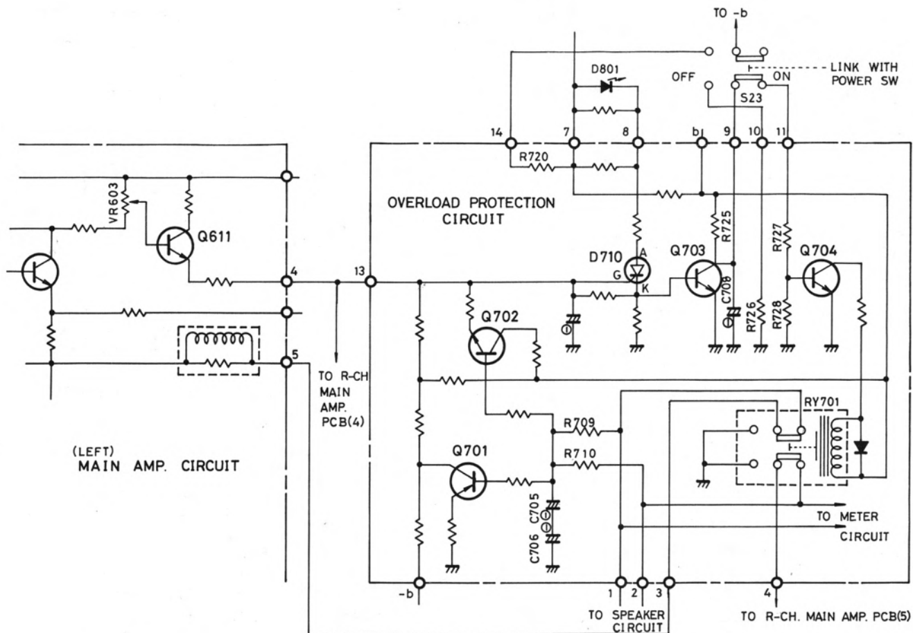
Fig. 6 OVERLOAD PROTECTION CIRCUIT
