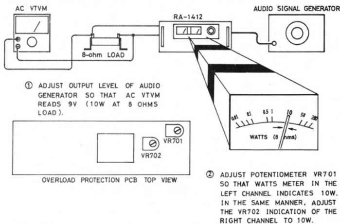
Fig. 5 WATTS METER CALIBRATION HOOK-UP
