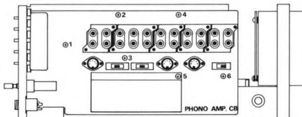
Fig. 1-6 RIGHT SIDE VIEW (2)
