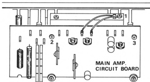
Fig. 1-9 CHASSIS TOP VIEW (MAIN AMP. PORTION)
