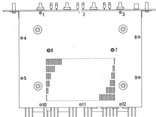
Fig. 1-2 BOTTOM VIEW
