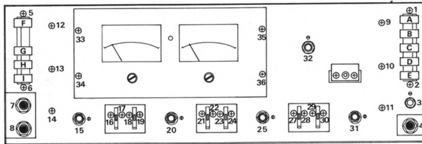
Fig. 1-4 FRONT CHASSIS
