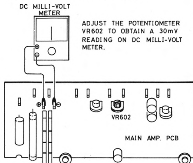
Fig.3 BIAS ADJUSTMENT HOOK-UP
