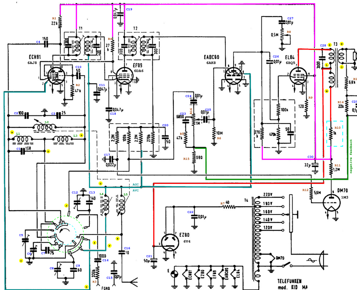
Radio Telefunken Kid R199, or Kid MA: original schematics with annotations.
