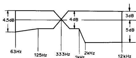
Fig. 8-4 Frequency response
