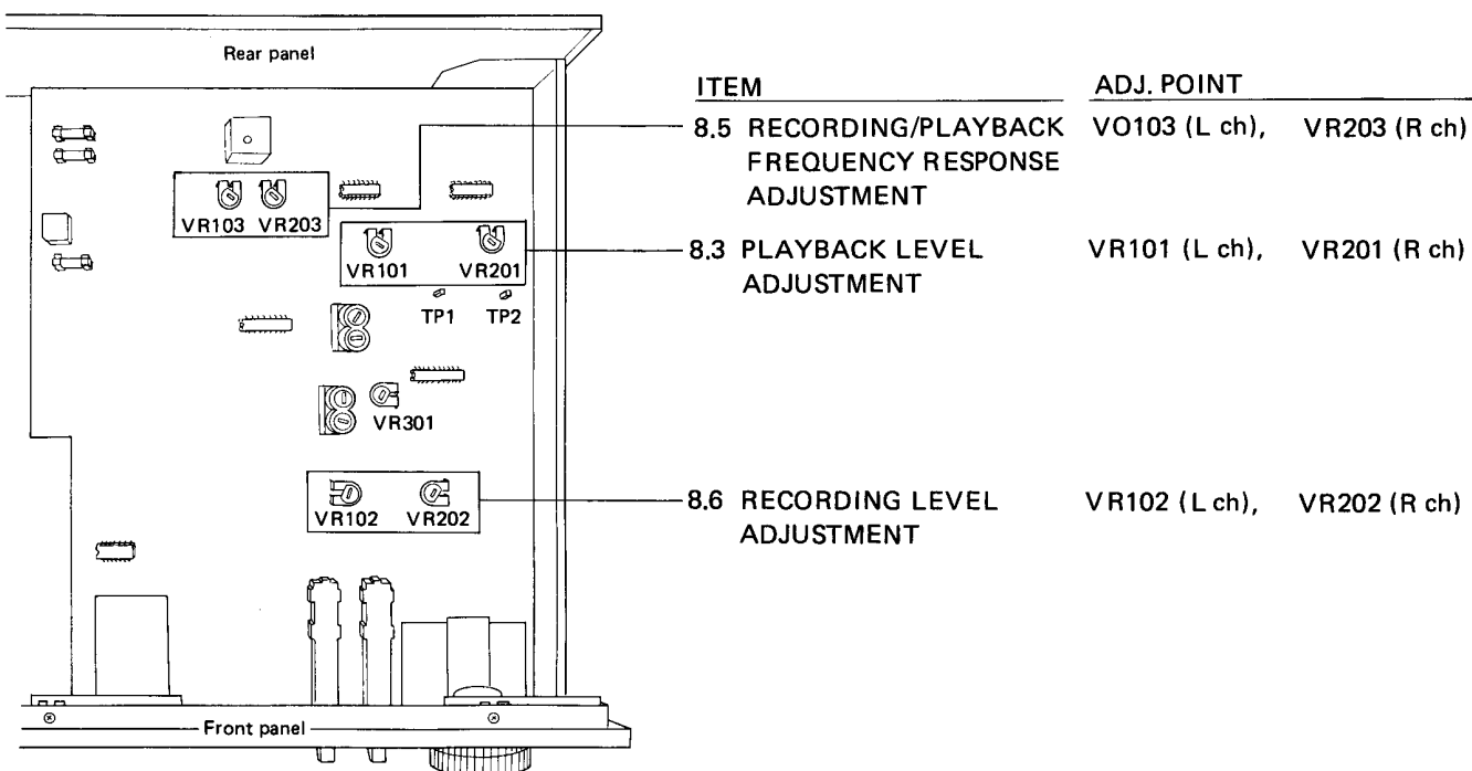
Fig. 8-3 Adjustment points
