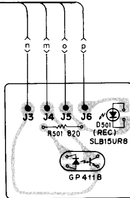
SENSOR Ass'y RWX-402
