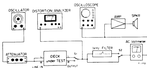
Fig. 3-2 Basic connection
