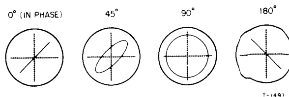
Fig. 3-5 Confirming phase relationship
