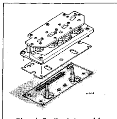
Fig. 4-7 Head Assembly
