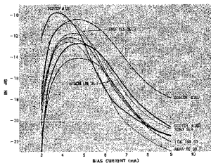
Fig. 7-9 Bias Current Characteristic
