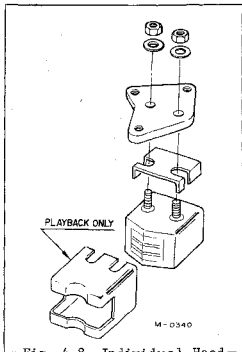
Fig. 4-8 Individual Head
