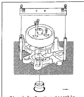
Fig. 4-5 Capstan Assembly
