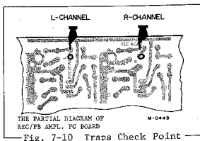
Fig. 7-10 Traps Check Point
