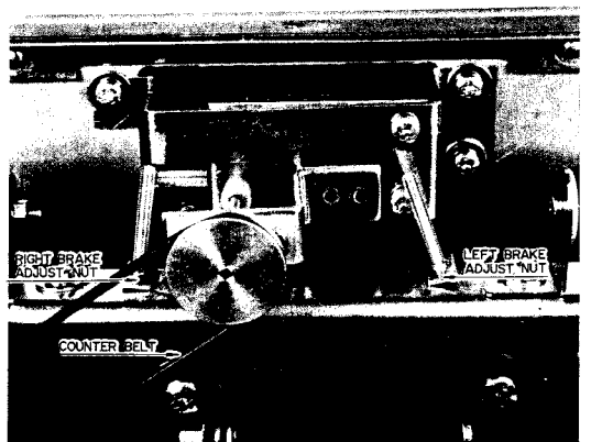
Fig. 6-5 Adjustable Location -Brake-
