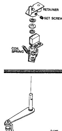
Fig. 4-7 Tension Arm -Right-
