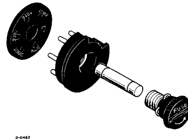
Fig. 6-7 voltage conversion
