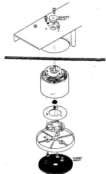
Fig. 4-4 Reel Motor Removal
