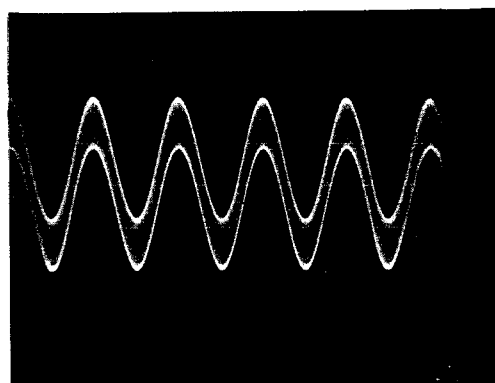
Fig. 7-7 Bias Leakage
