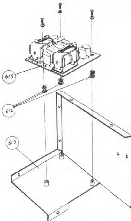
A-4000S LEFT CHASSIS ASS'Y, EXPLODED VIEW
