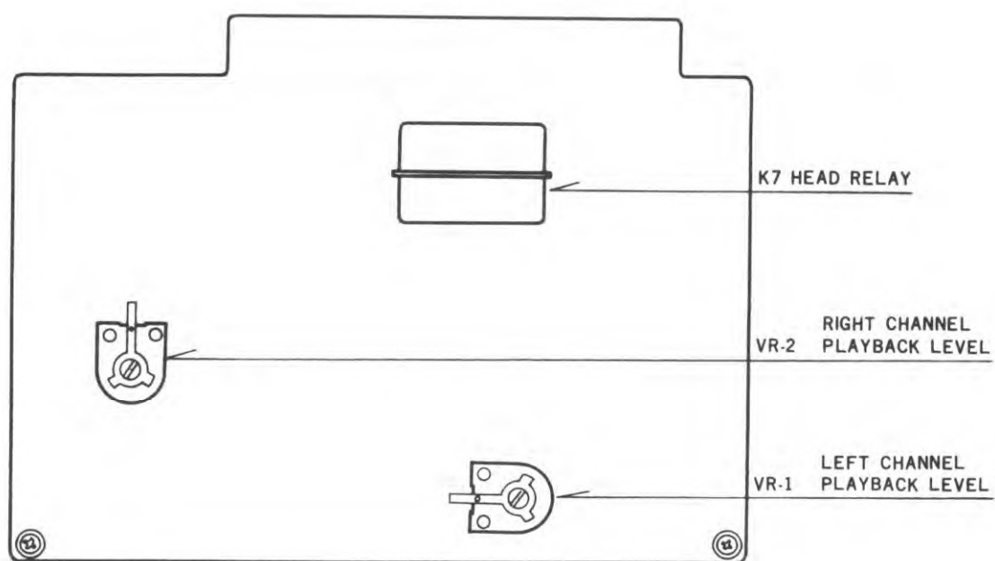
FIG.13 A-4000S PLAYBACK AMPLIFIER PRINTED BOARD ADJUSTABLE PARTS LOCATION (TOP VIEW)
