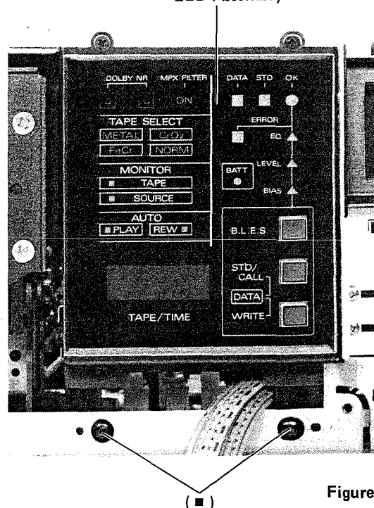
Counter &amp; LED Assembly
