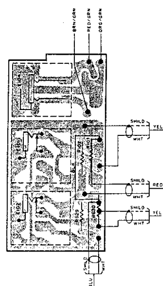
Bottom View
