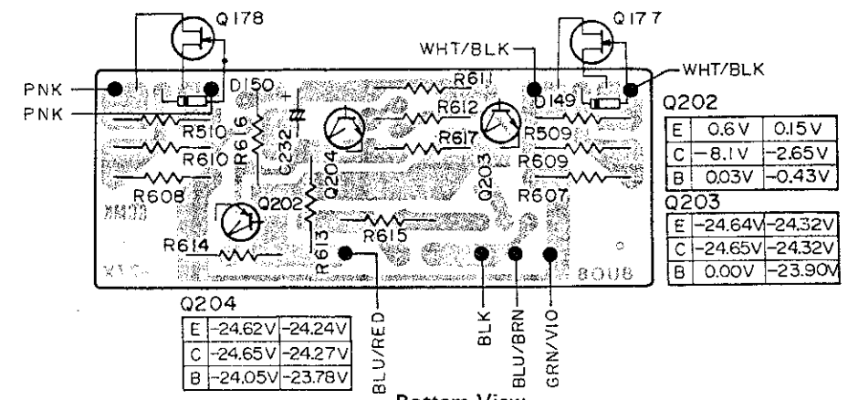
Bottom View
