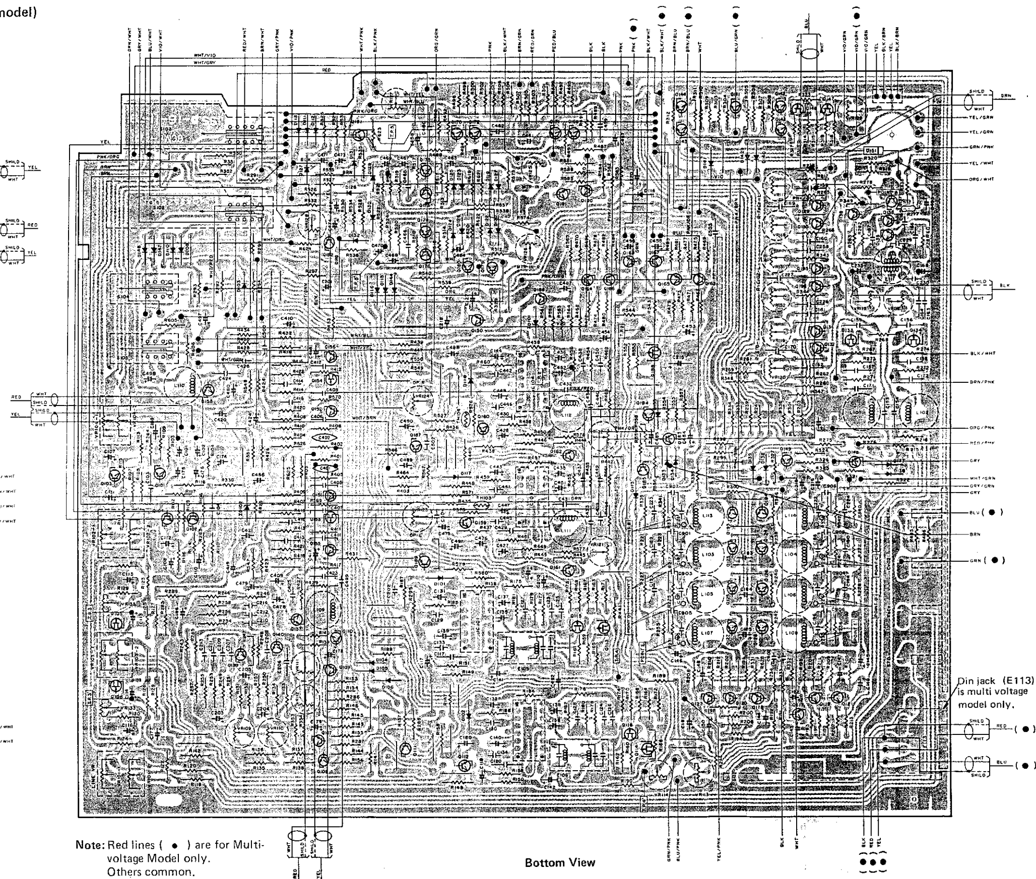
Bottom View
