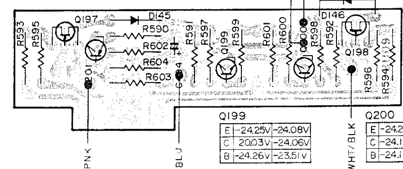
Bottom View
