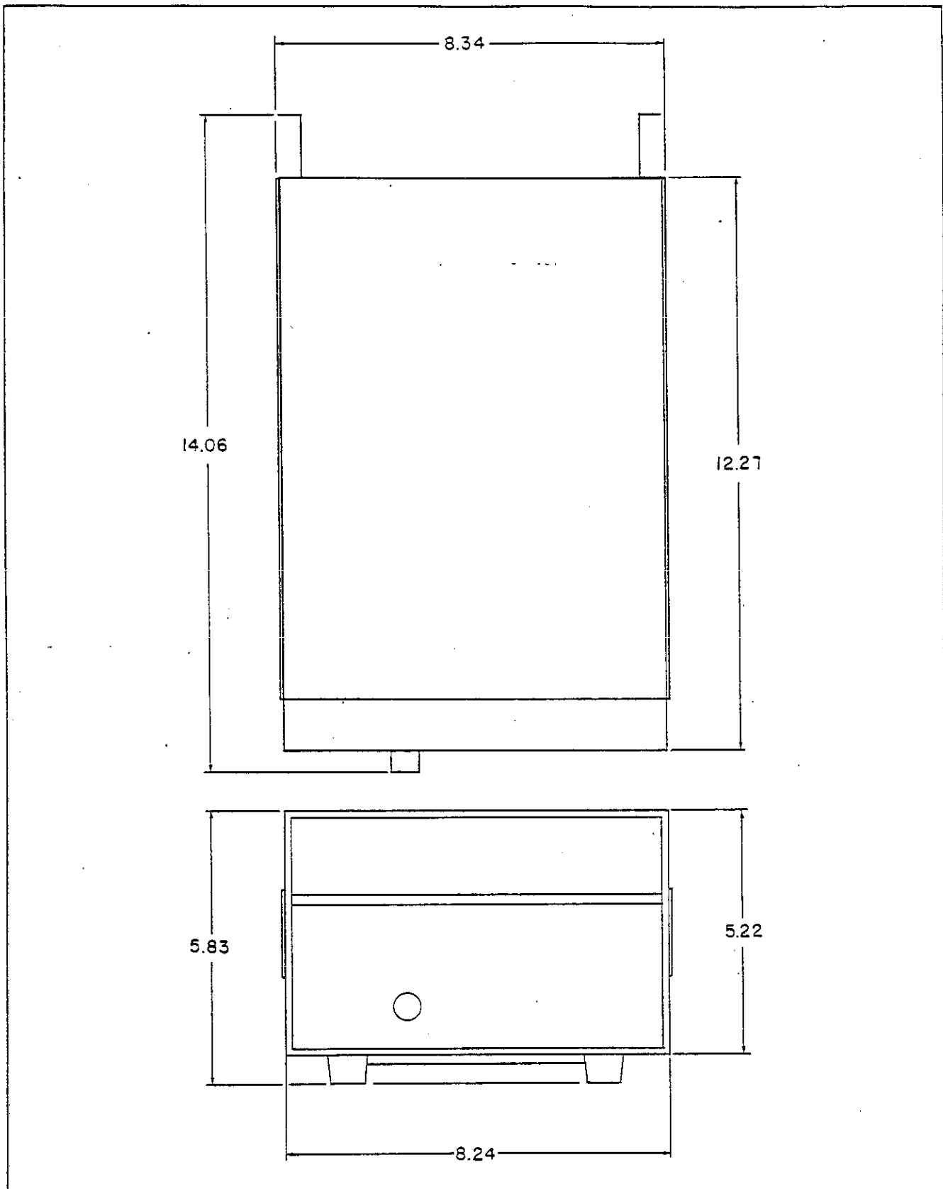
Figure 1-2 Outline Dimensions
