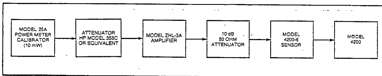
Figure 5-7. Test Setup for Determination of Attenuation Value
