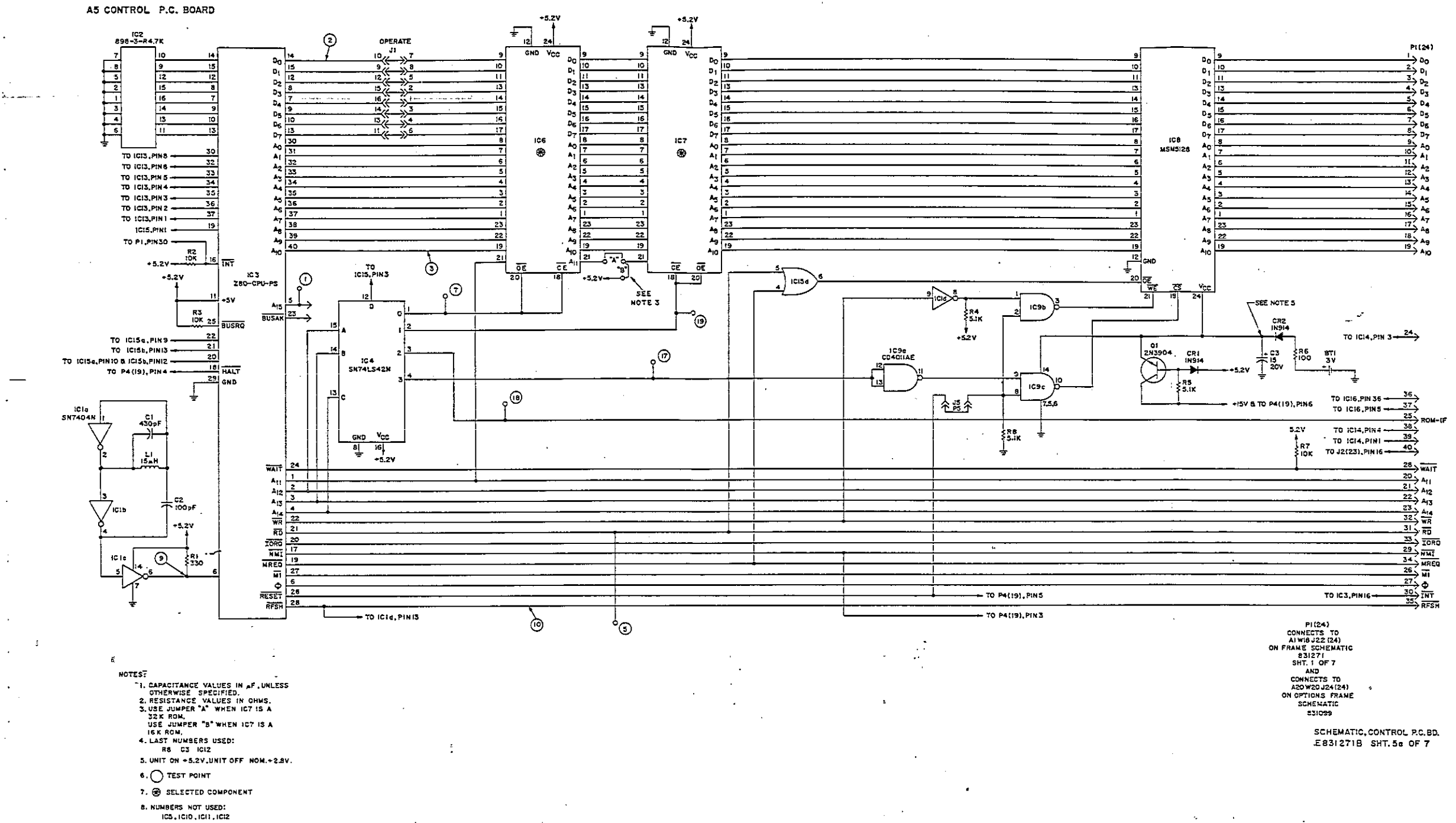
Figure 7-5 Control Board A5, Schematic Diagram (Sheet 2 of 2)
