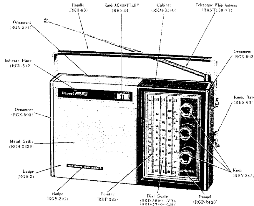
Fig. 11 Cabinet &amp; Appearance—Parts Identification
