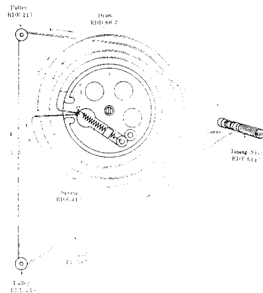
Fig. 12 Dial Cord Stringing Guide
