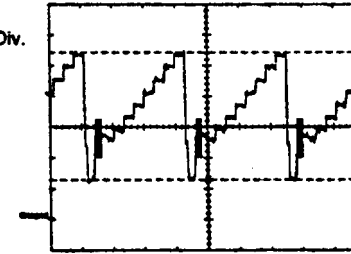
OSZ-24 960 mVss, 20 \mu s/Div. MC 44007 Pin 37
