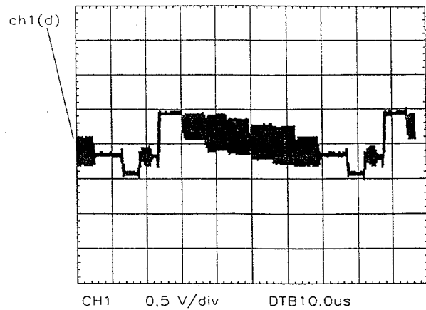
Pin 7 IC903 with signal video from Tuner
