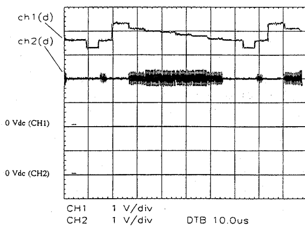
CH1 Pin 7 CI903 CH2 Pin 6 CI903 (with signal input SVHS)
