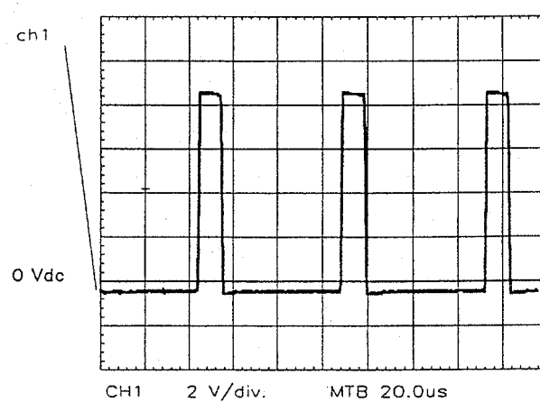
Pin 41 IC903 (Flyback)
