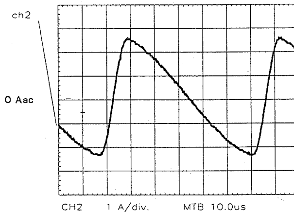
Vertical yoke current
