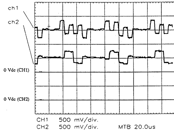
CH1 Pin 29 CI903 (B-Y) CH2 Pin 30 CI903 (R-Y)
