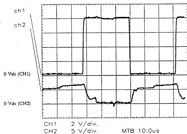
Horizontal: CH1 Pin 40 CI903 CH2 TP19
