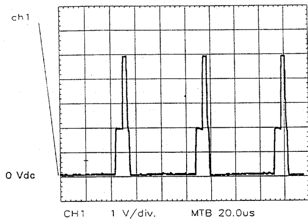
Pin 39 IC903 (Super-sandcastle)
