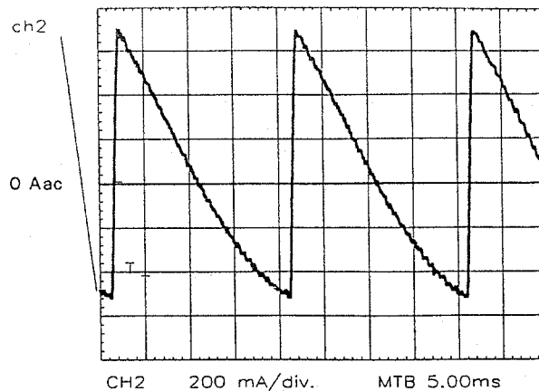
Horizontal yoke current
