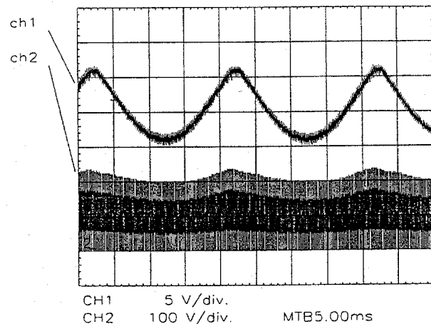
E/W: CH1 Pin 11 CI601 CH2 wave form on D305
