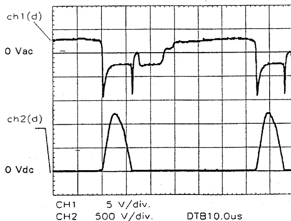
Horizontal: CH1 Base T301 CH2 Collector T301
